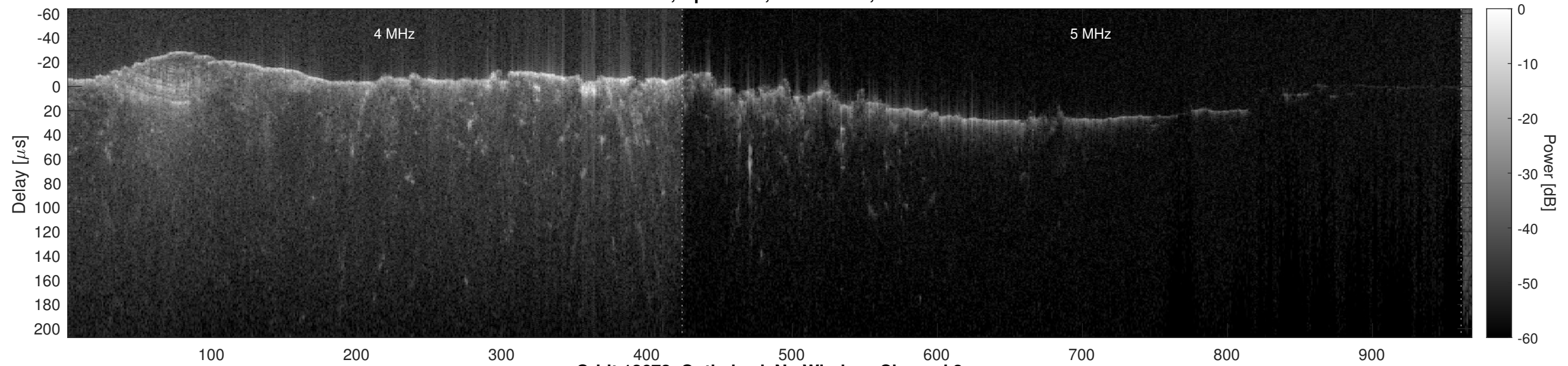
Orbit 12672, Optimized, No Window, Channel 2
