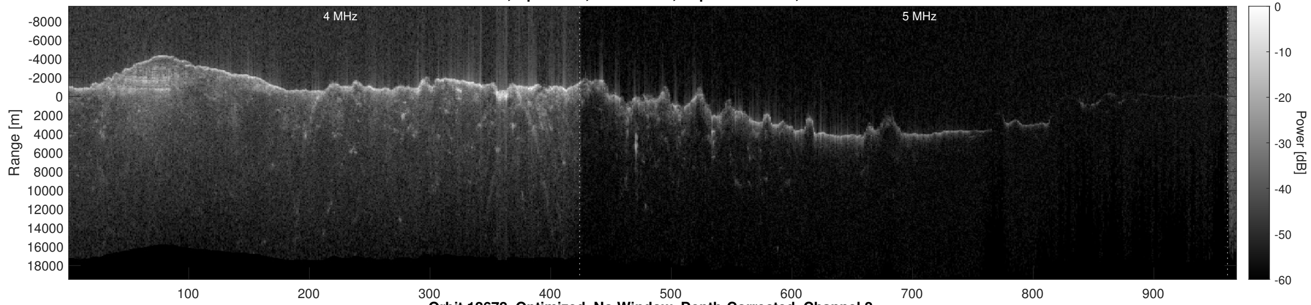
Orbit 12672, Optimized, No Window, Depth-Corrected, Channel 2
