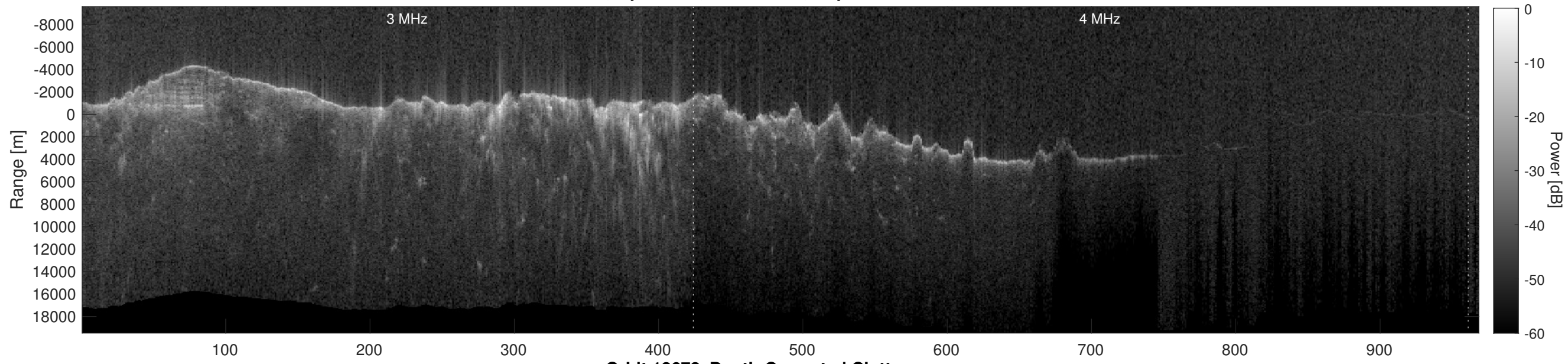
Orbit 12672, Depth-Corrected Cluttergram
