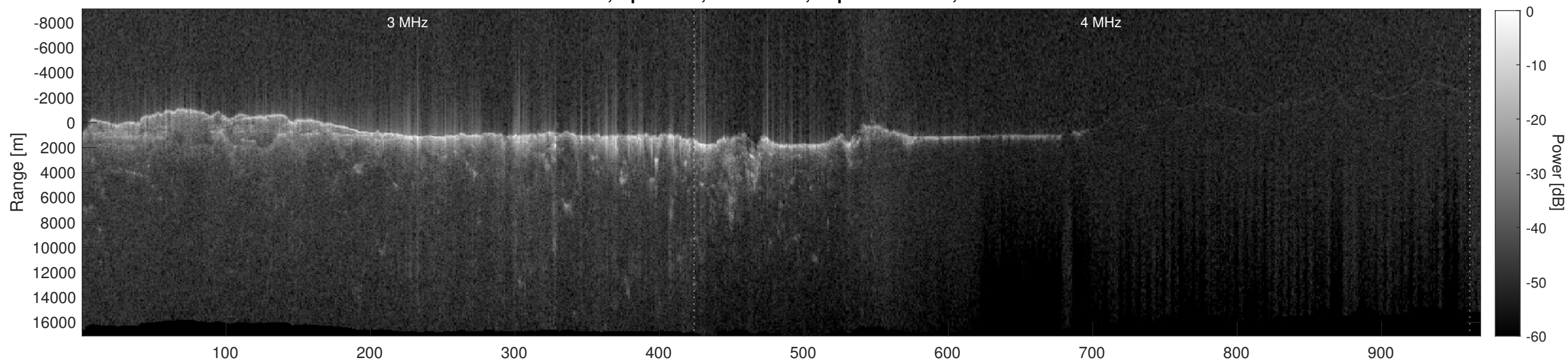
Orbit 12674, Depth-Corrected Cluttergram
