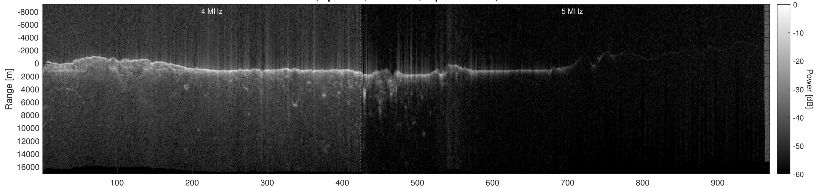
Orbit 12674, Optimized, No Window, Depth-Corrected, Channel 2
