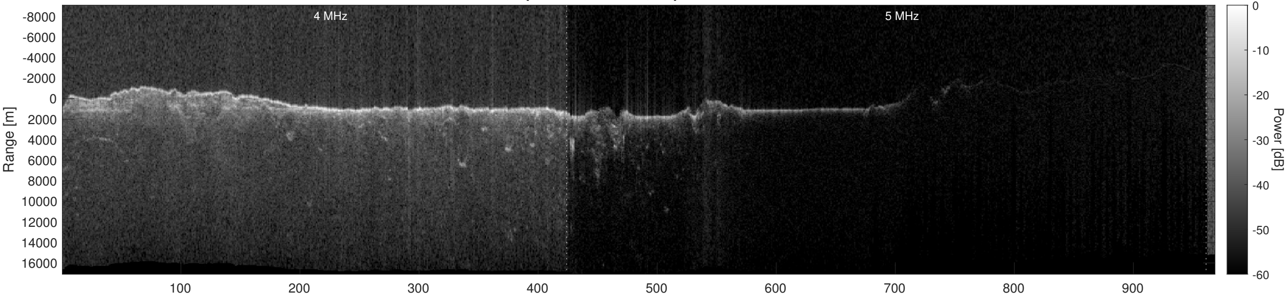
Orbit 12674, Optimized, Window, Depth-Corrected, Channel 2
