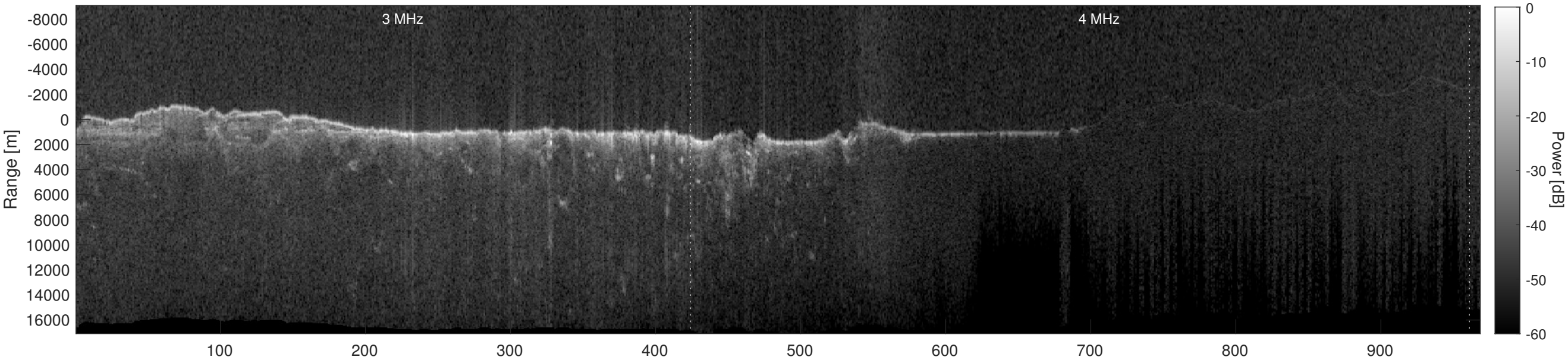
Orbit 12674, Depth-Corrected Cluttergram
