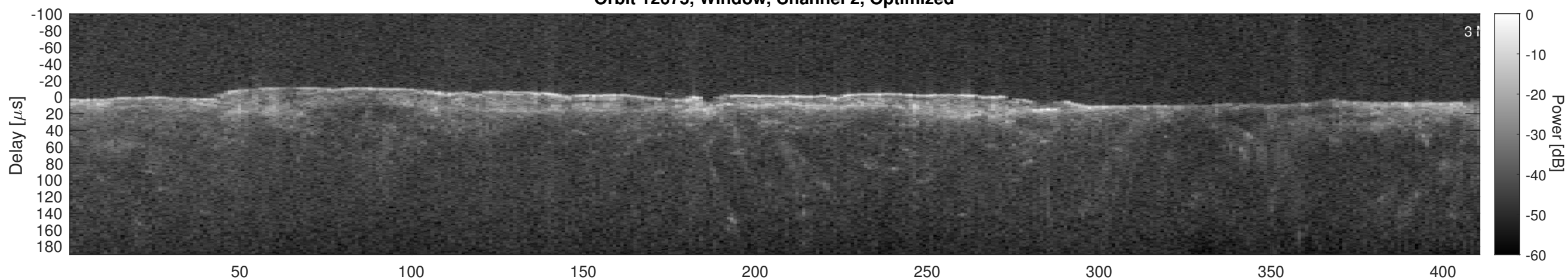
Orbit 12675, Cluttergram
