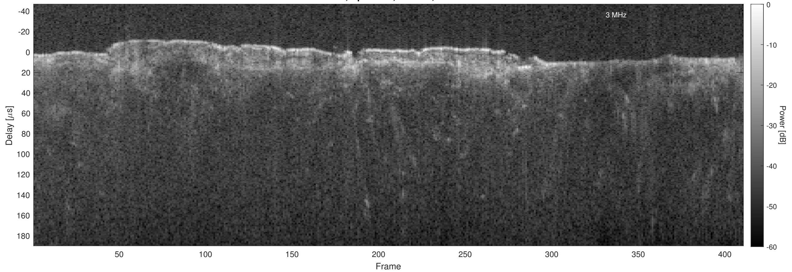
Orbit 12675, Optimized, Window, Channel 2
