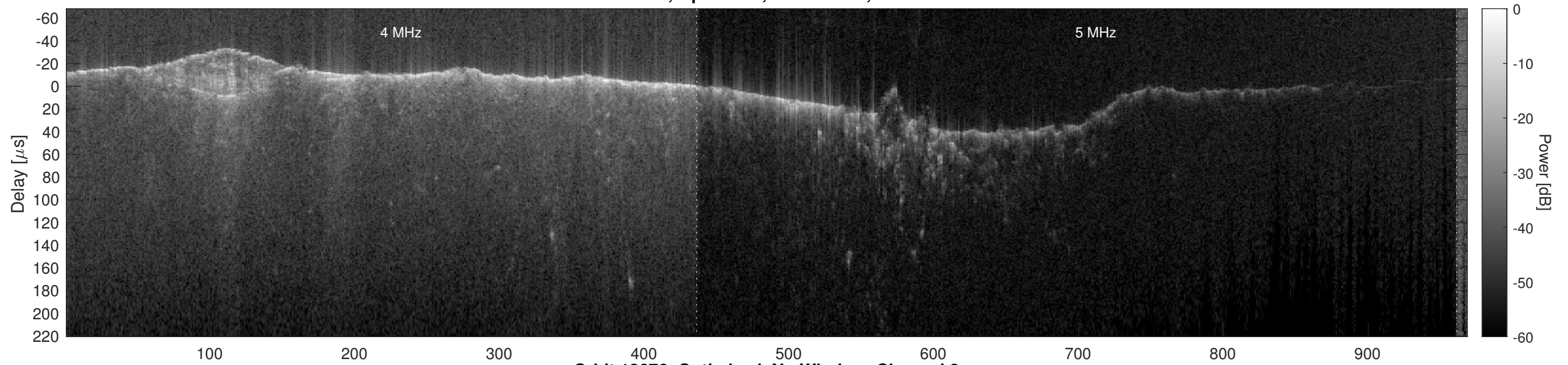
Orbit 12676, Optimized, No Window, Channel 2
