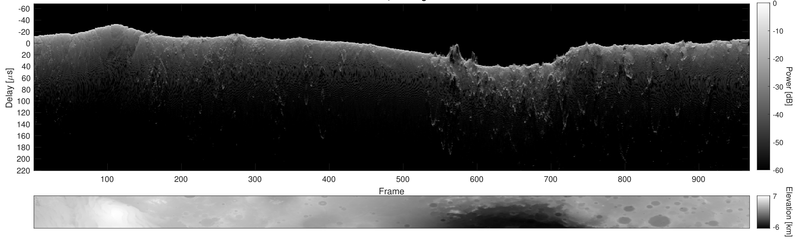
Orbit 12676, Cluttergram
