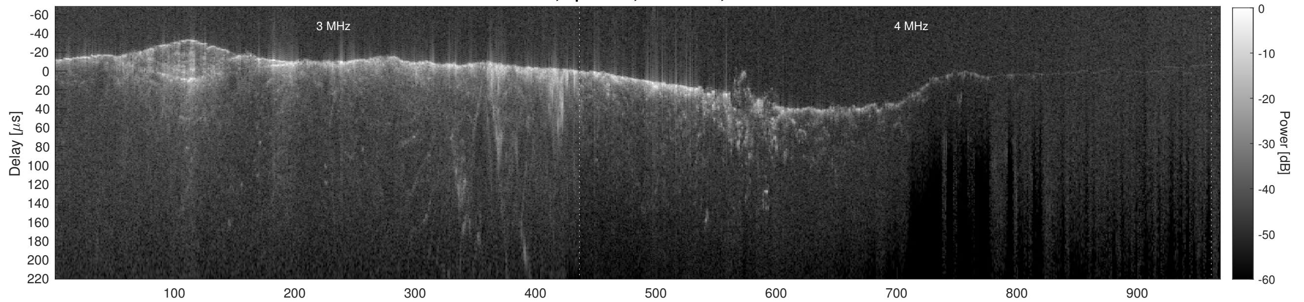
Orbit 12676, Cluttergram
