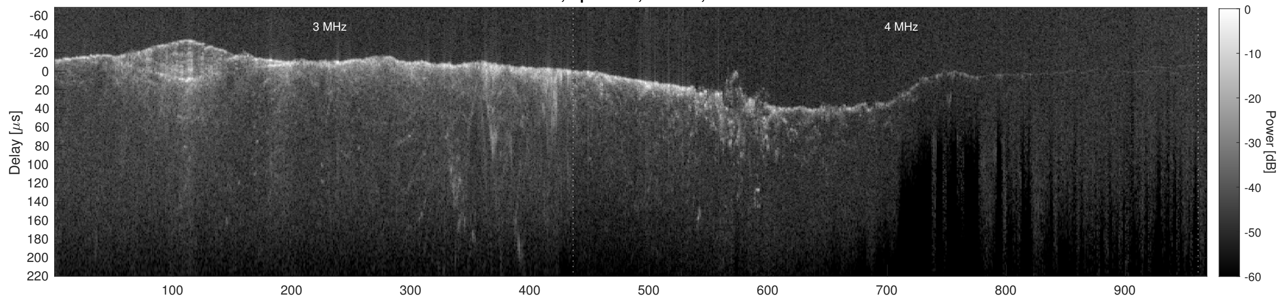
Orbit 12676, Cluttergram
