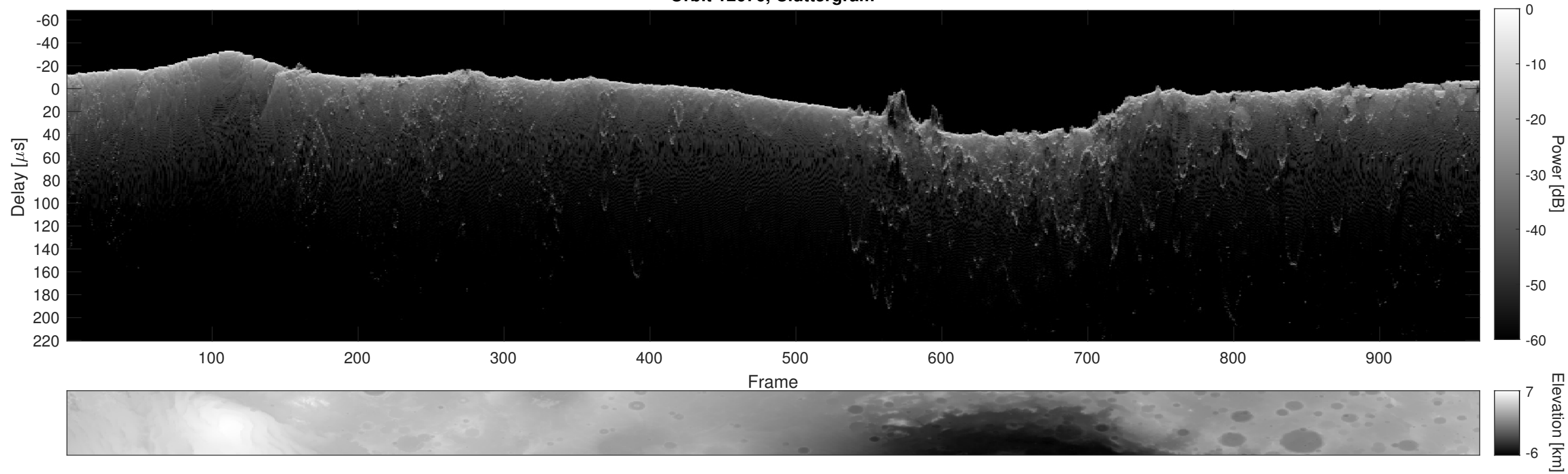
Orbit 12676, Cluttergram
