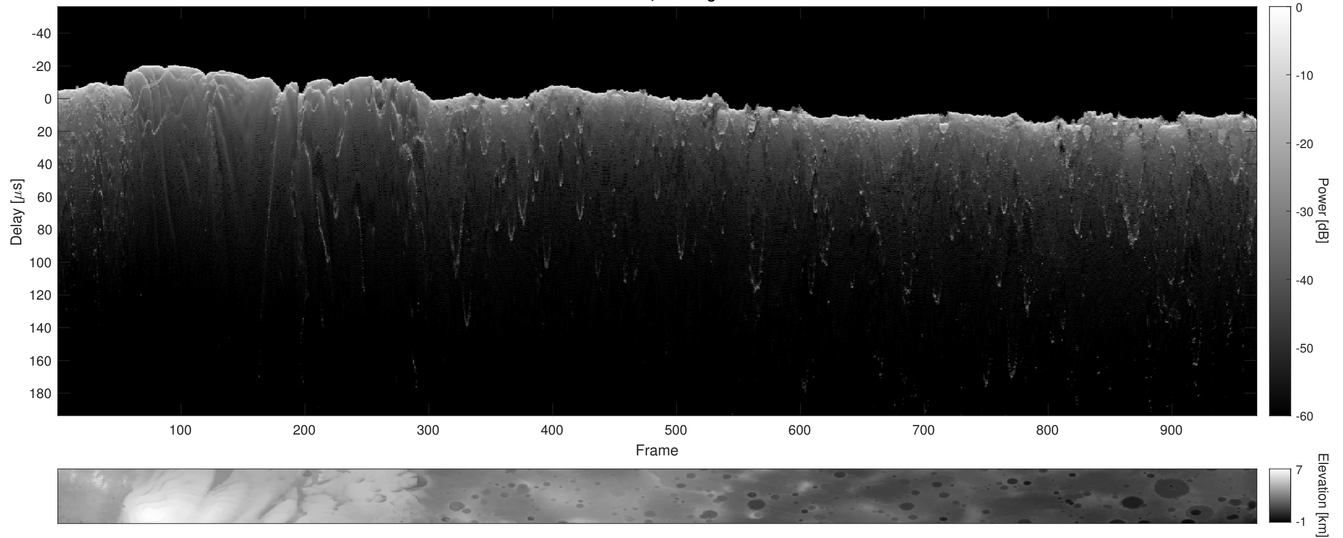
Orbit 12682, Cluttergram
