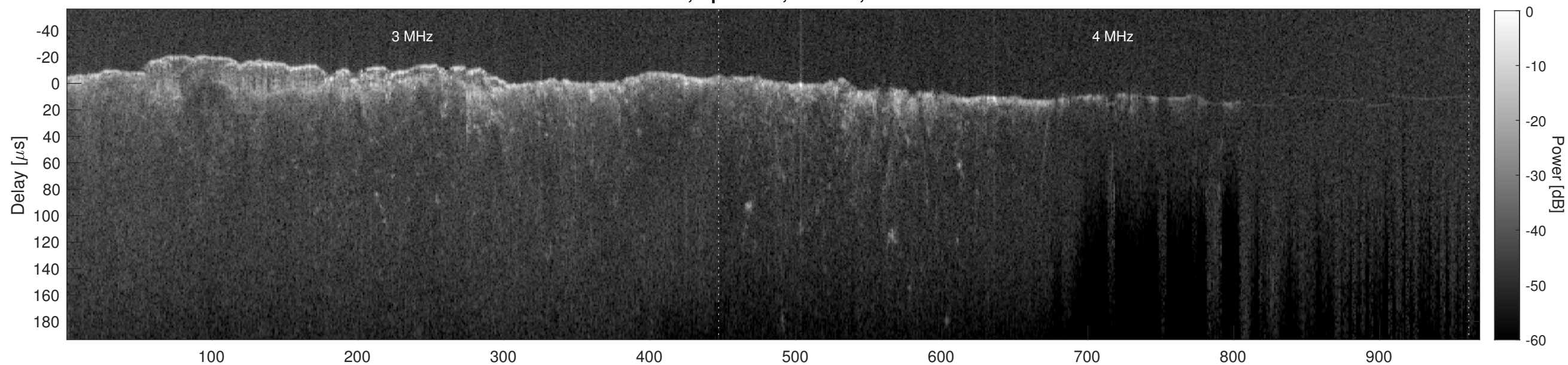
Orbit 12682, Cluttergram
