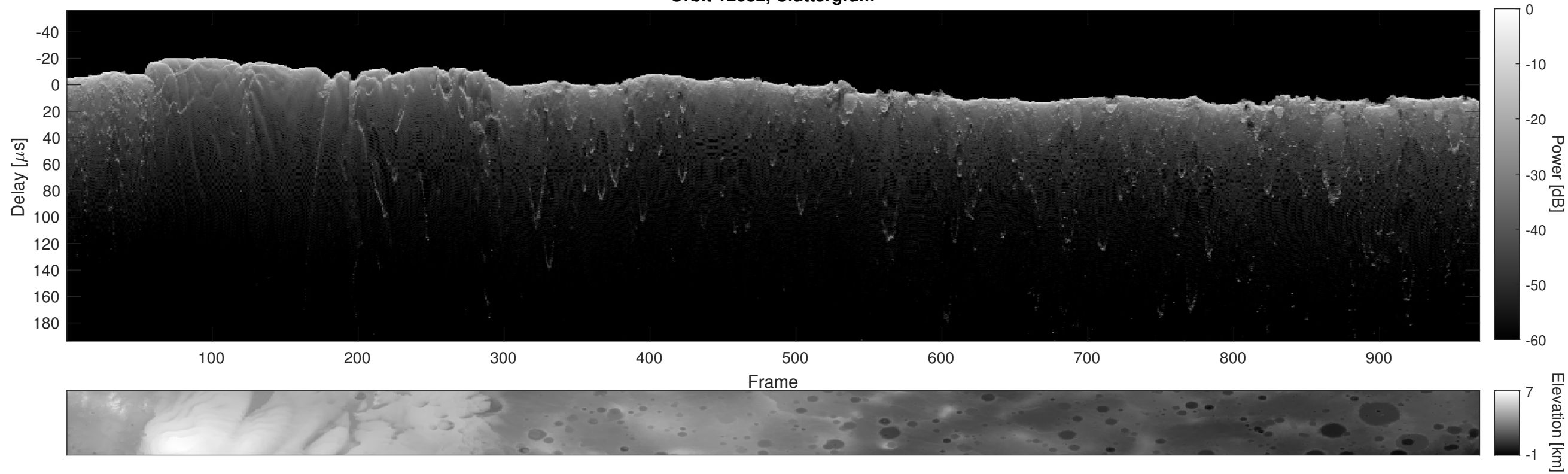
Orbit 12682, Cluttergram
