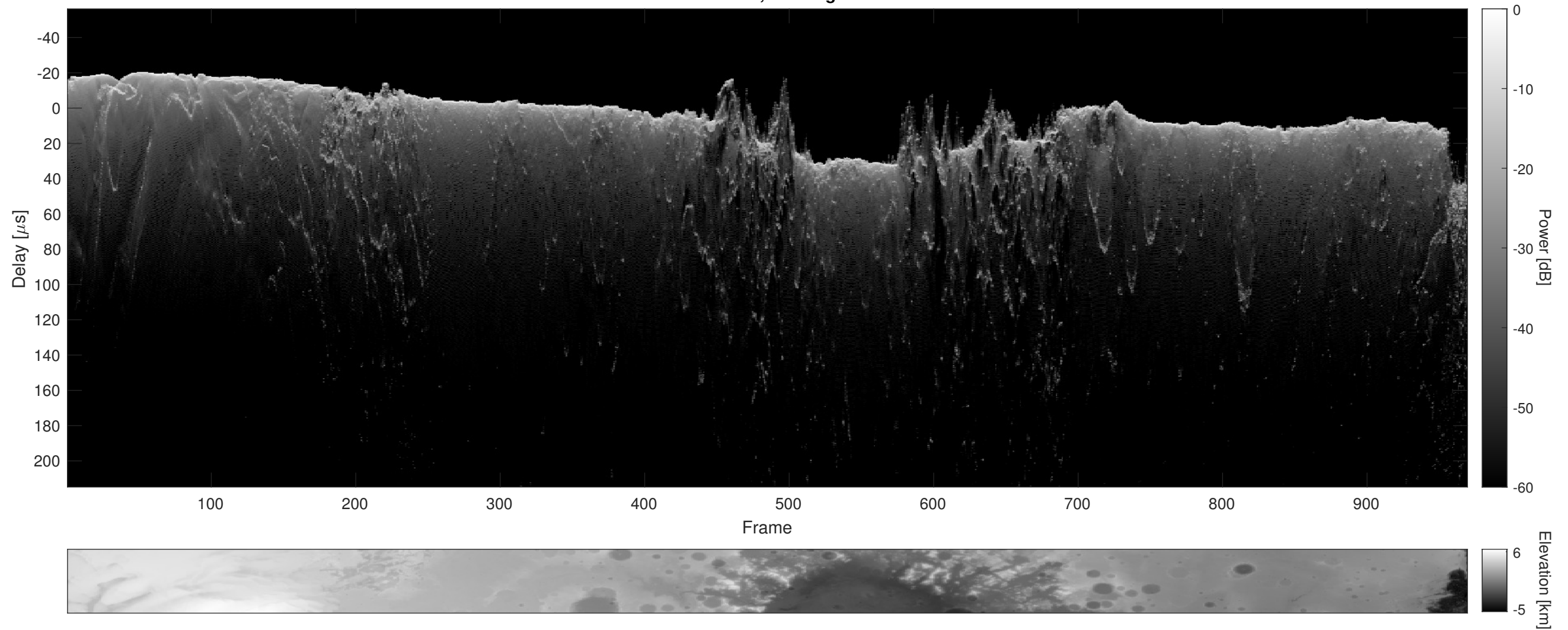
Orbit 12684, Cluttergram
