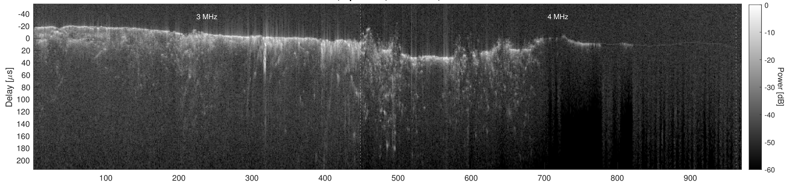
Orbit 12684, Cluttergram
