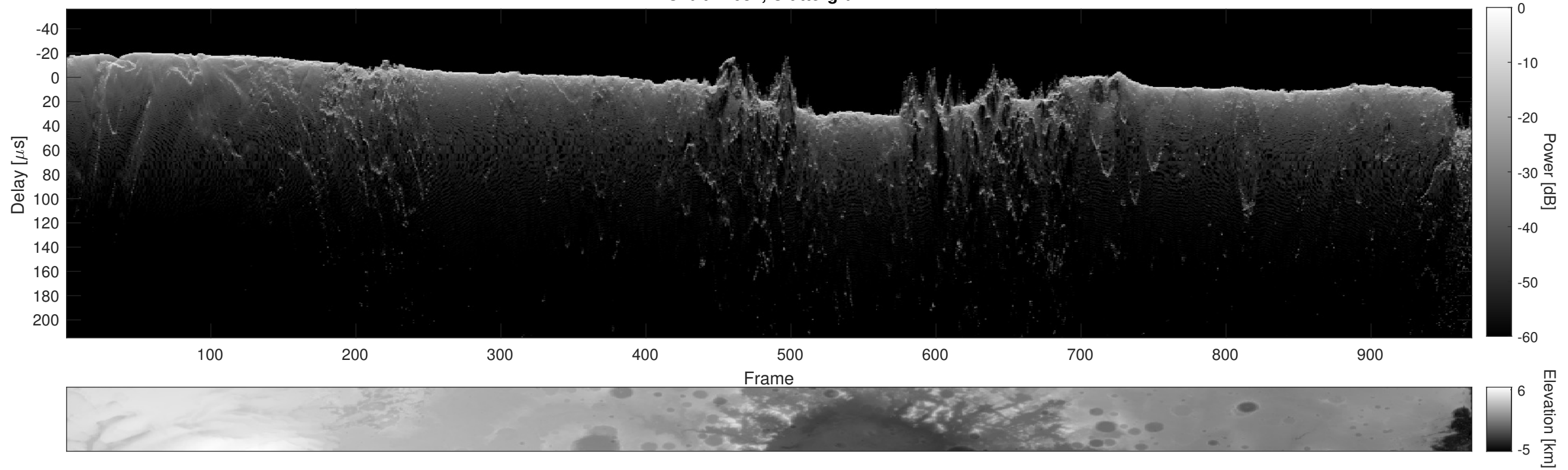
Orbit 12684, Cluttergram
