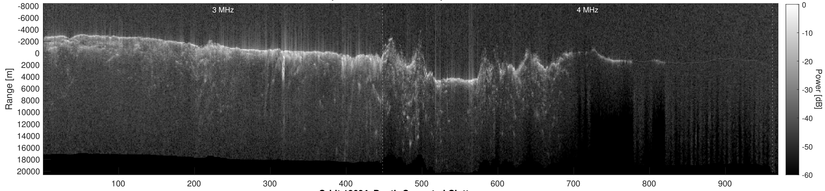
Orbit 12684, Depth-Corrected Cluttergram
