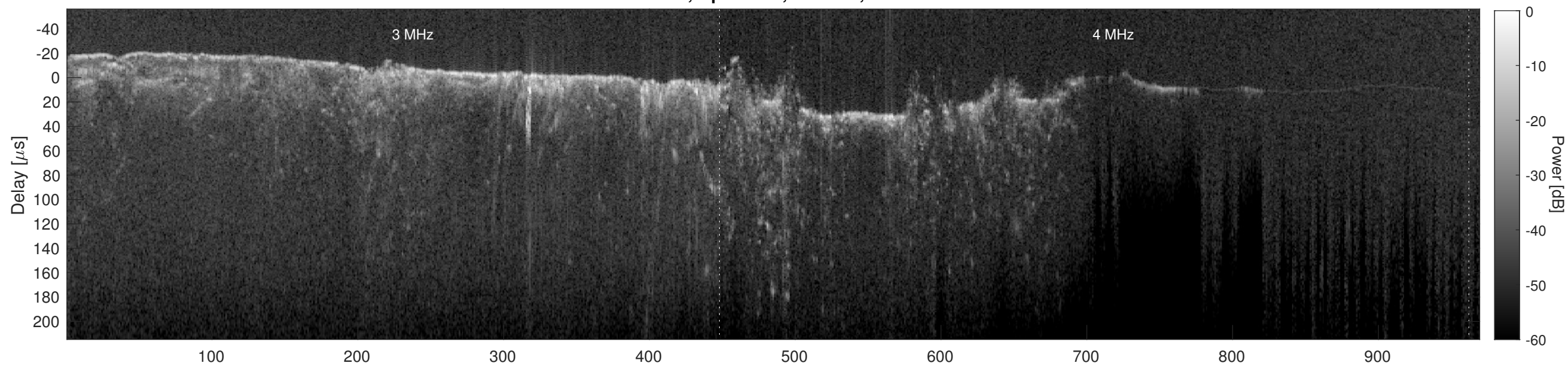
Orbit 12684, Cluttergram
