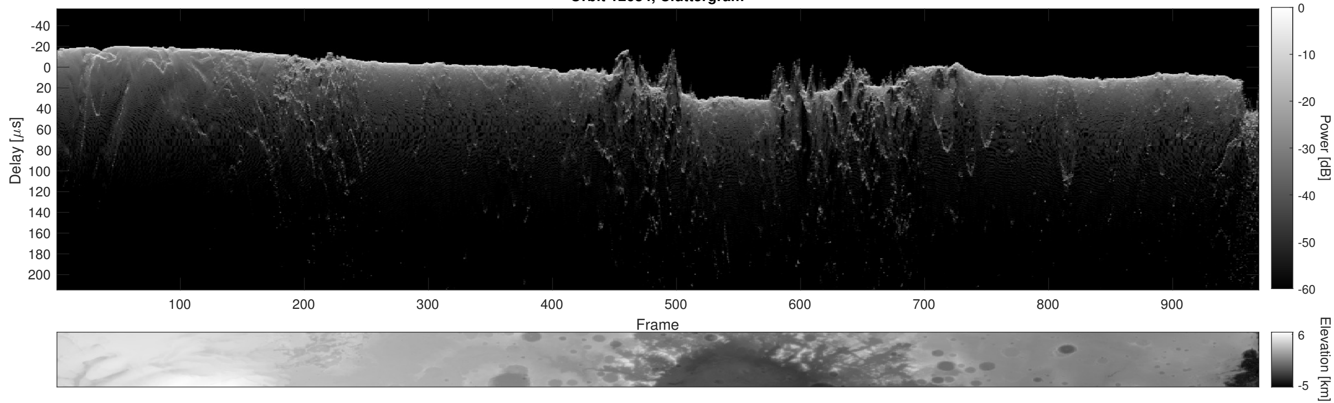
Orbit 12684, Cluttergram
