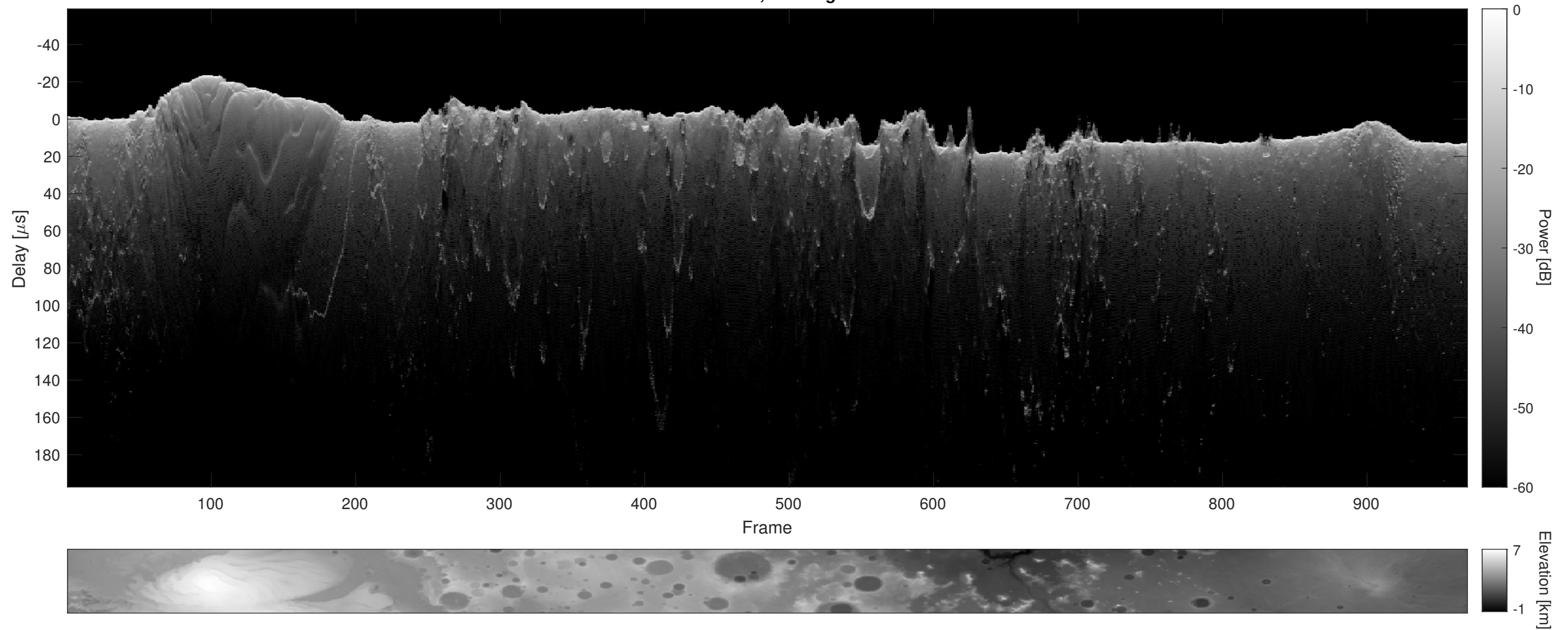
Orbit 12686, Cluttergram
