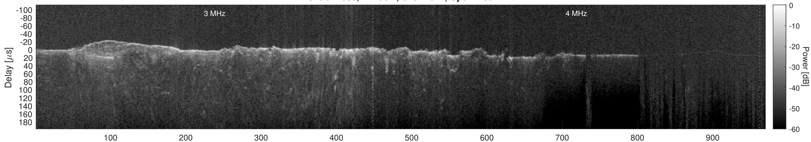
Orbit 12686, Cluttergram
