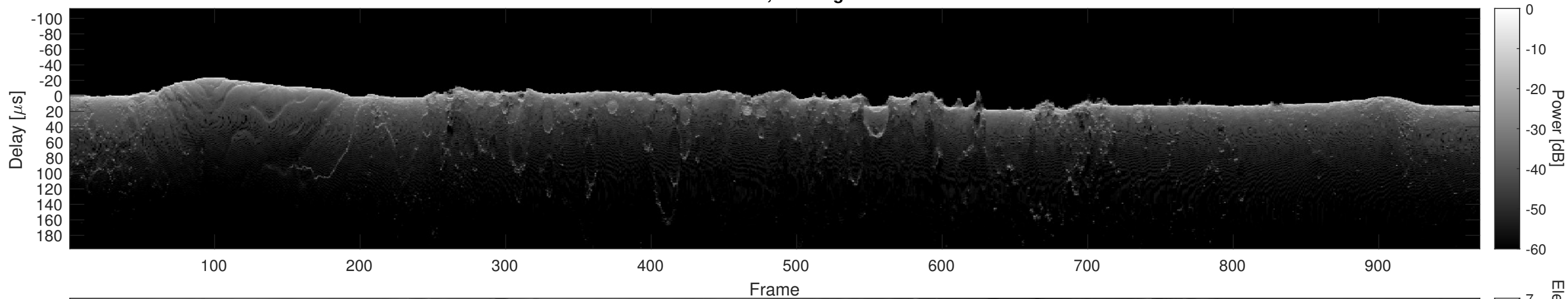
Orbit 12686, Cluttergram
