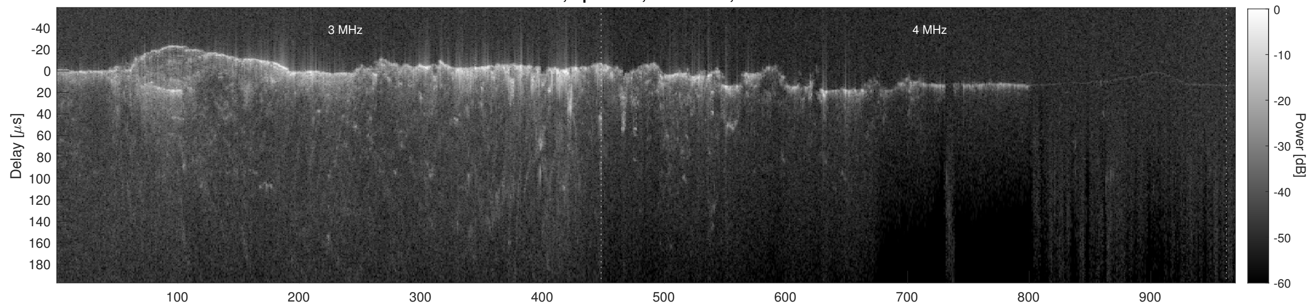
Orbit 12686, Cluttergram
