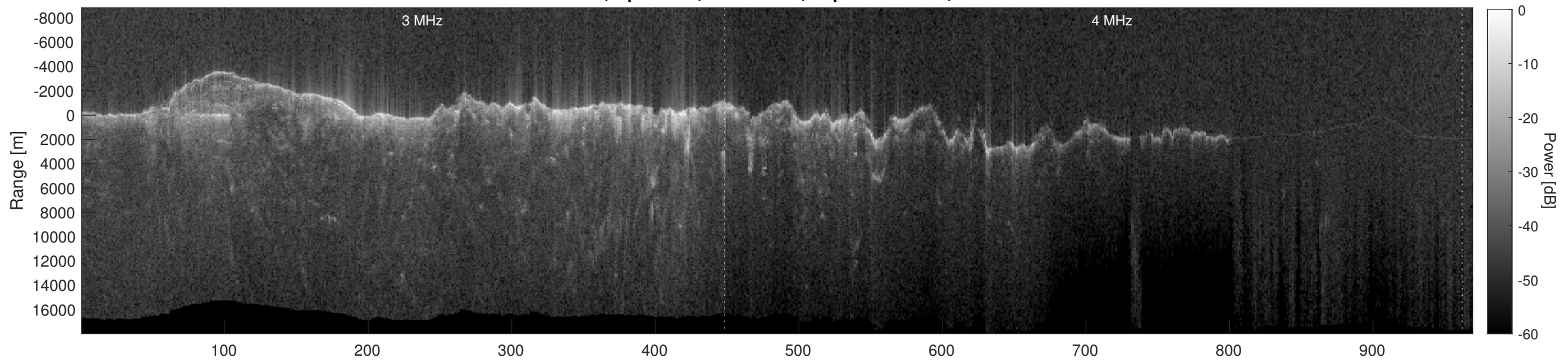
Orbit 12686, Depth-Corrected Cluttergram
