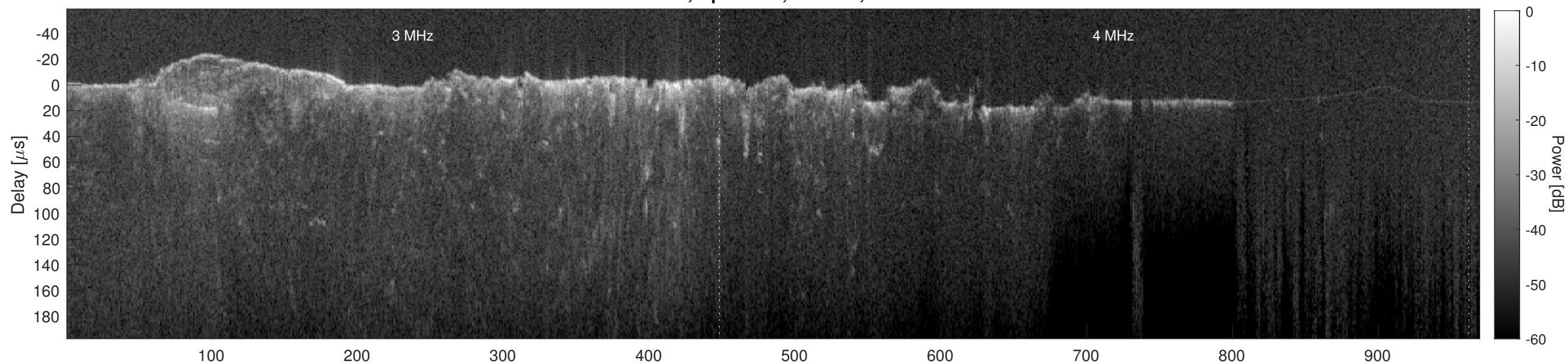
Orbit 12686, Cluttergram
