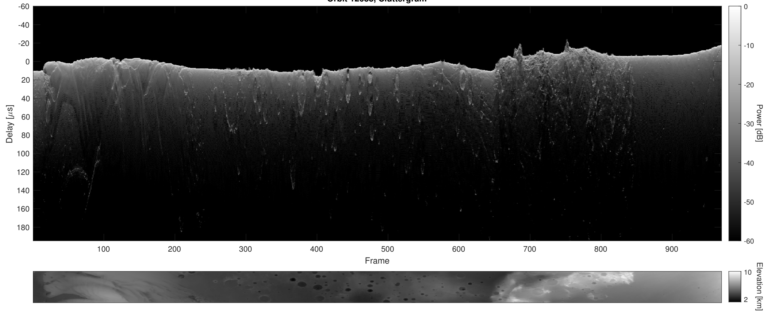
Orbit 12688, Cluttergram
