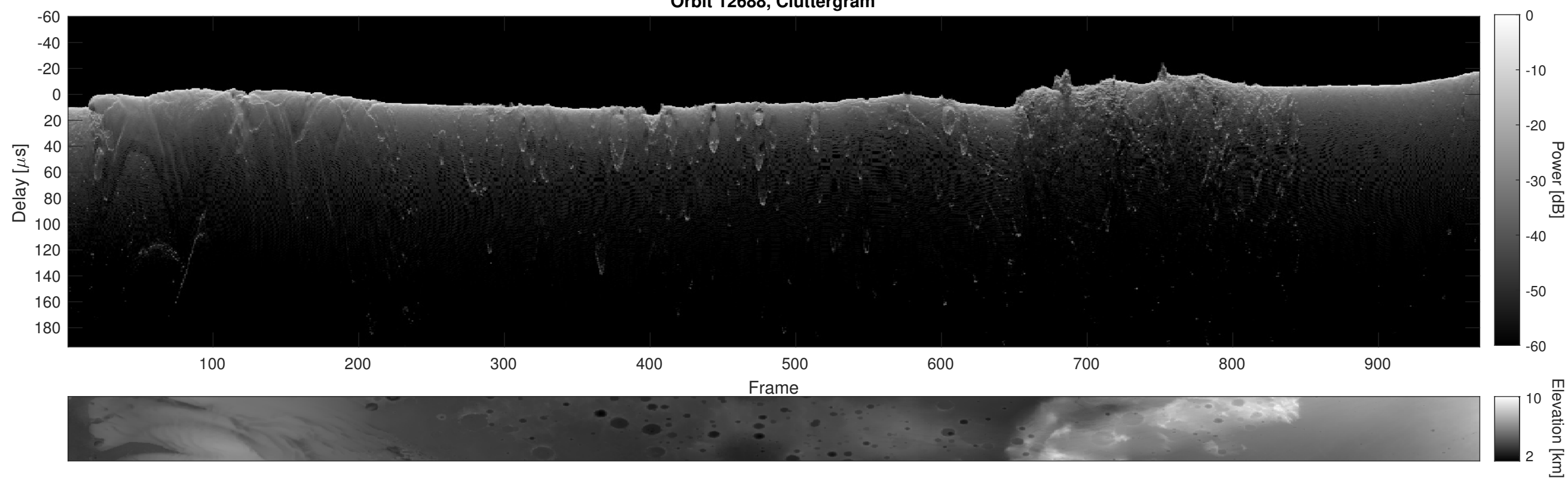
Orbit 12688, Cluttergram
