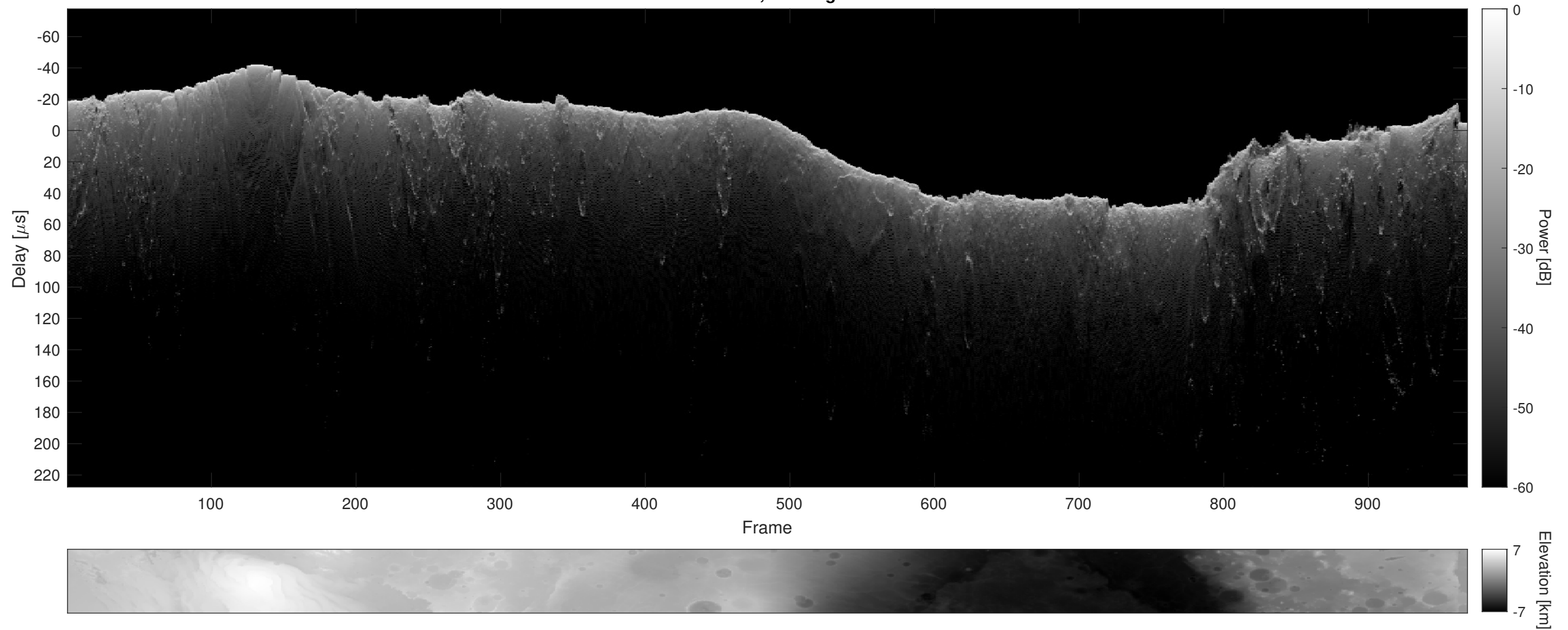
Orbit 12690, Cluttergram
