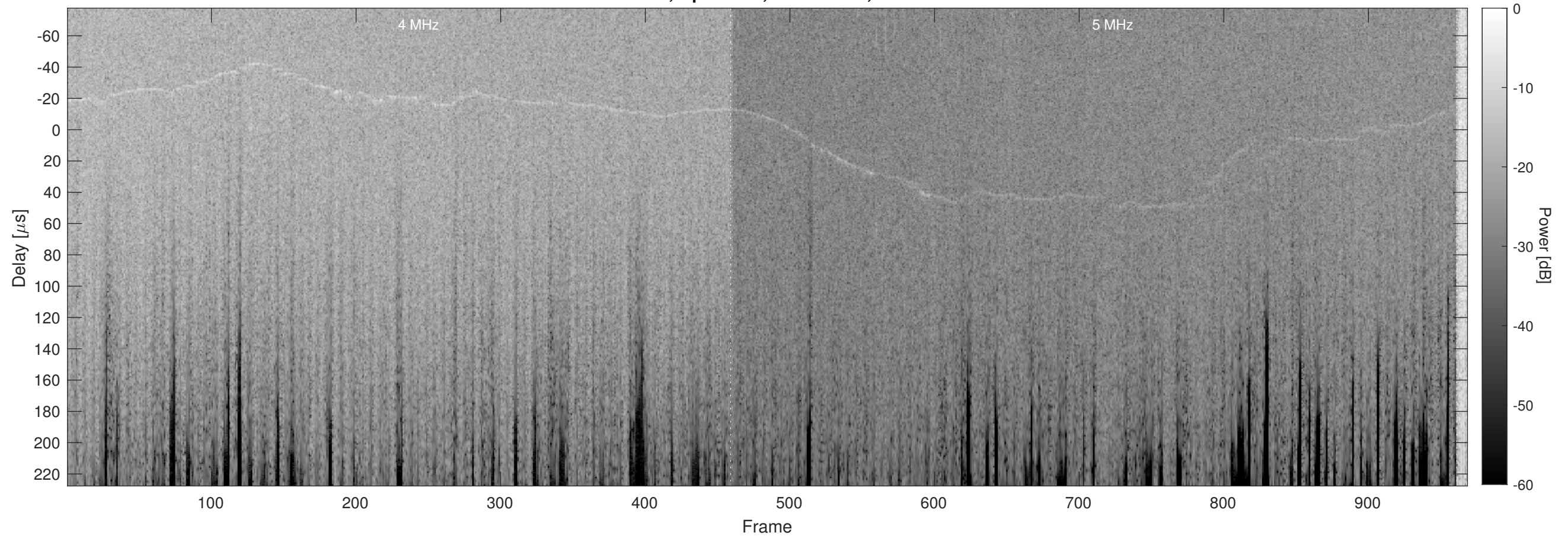
Orbit 12690, Optimized, No Window, Channel 2
