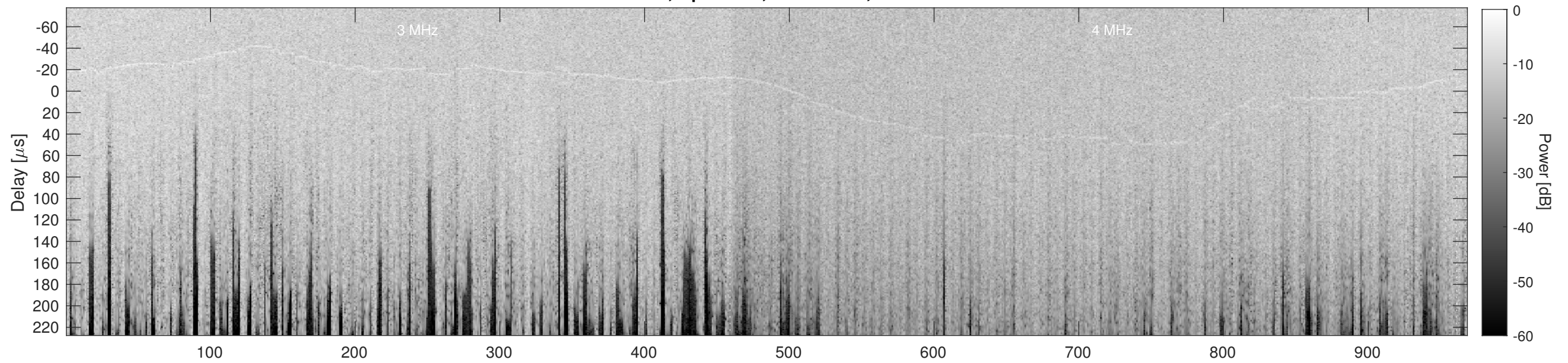
Orbit 12690, Cluttergram
