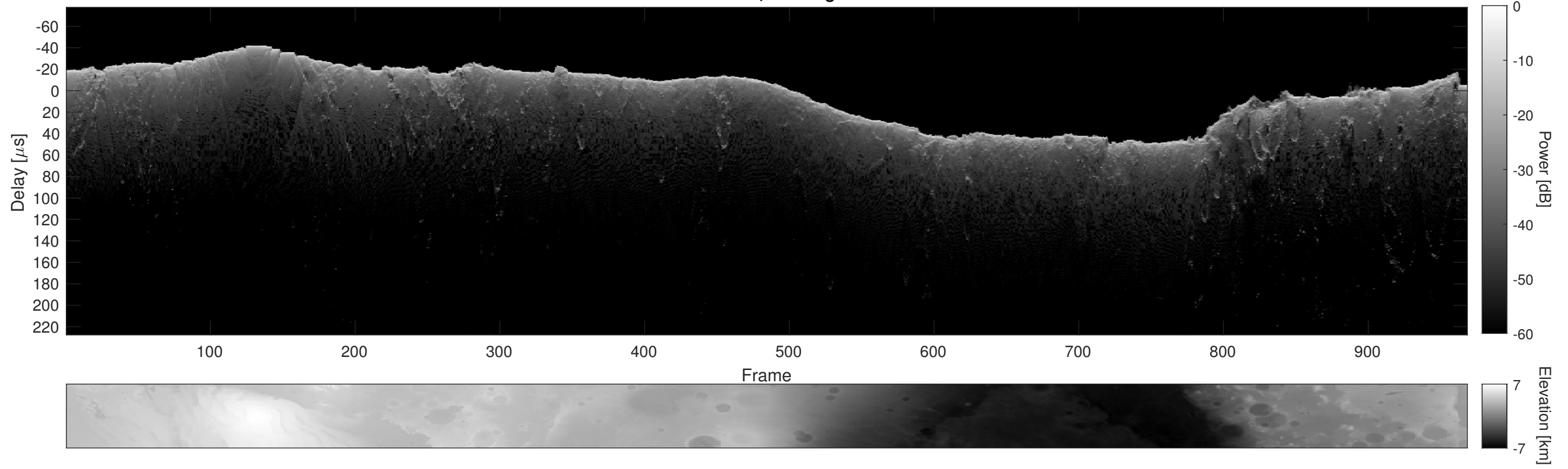
Orbit 12690, Cluttergram
