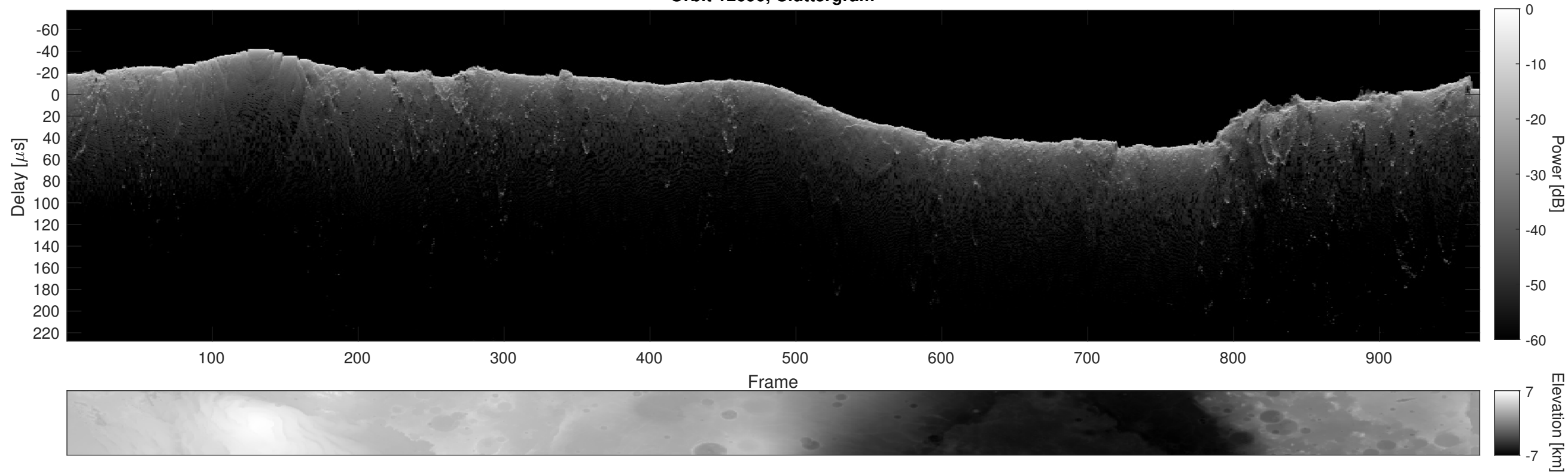
Orbit 12690, Cluttergram
