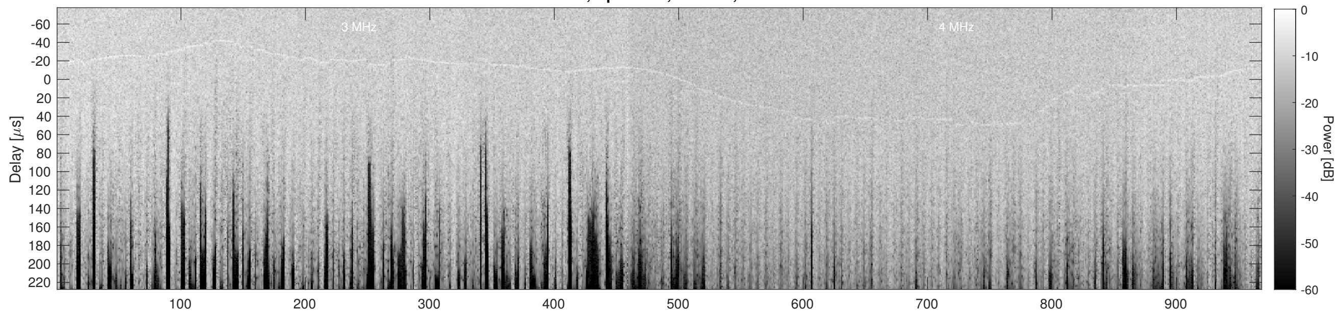
Orbit 12690, Cluttergram
