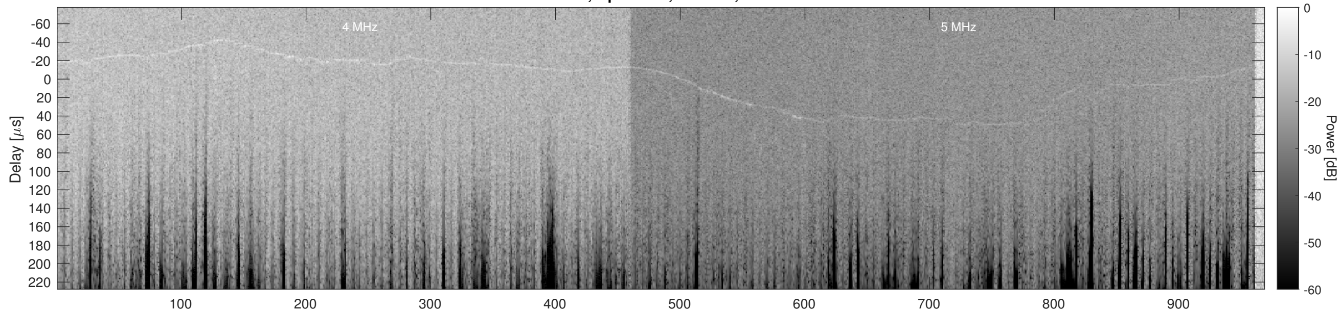
Orbit 12690, Optimized, Window, Channel 2
