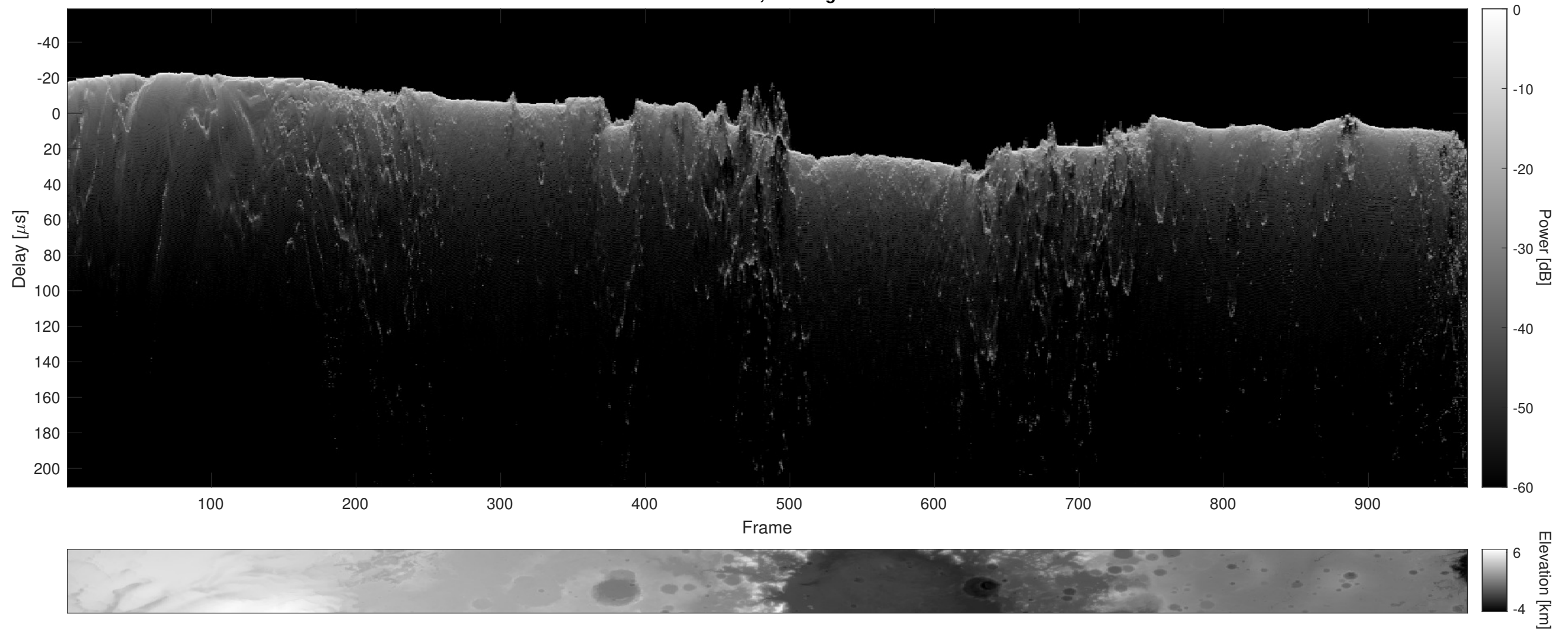
Orbit 12691, Cluttergram
