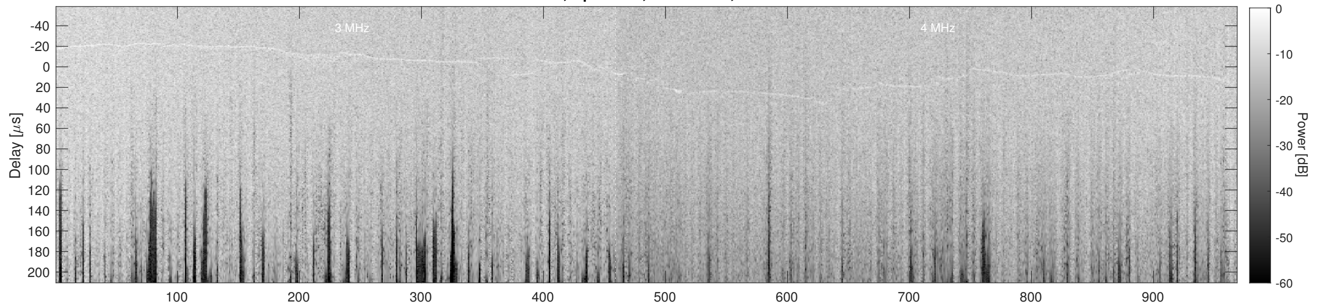
Orbit 12691, Cluttergram
