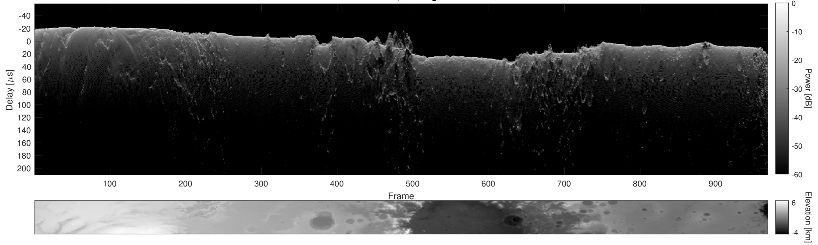
Orbit 12691, Cluttergram
