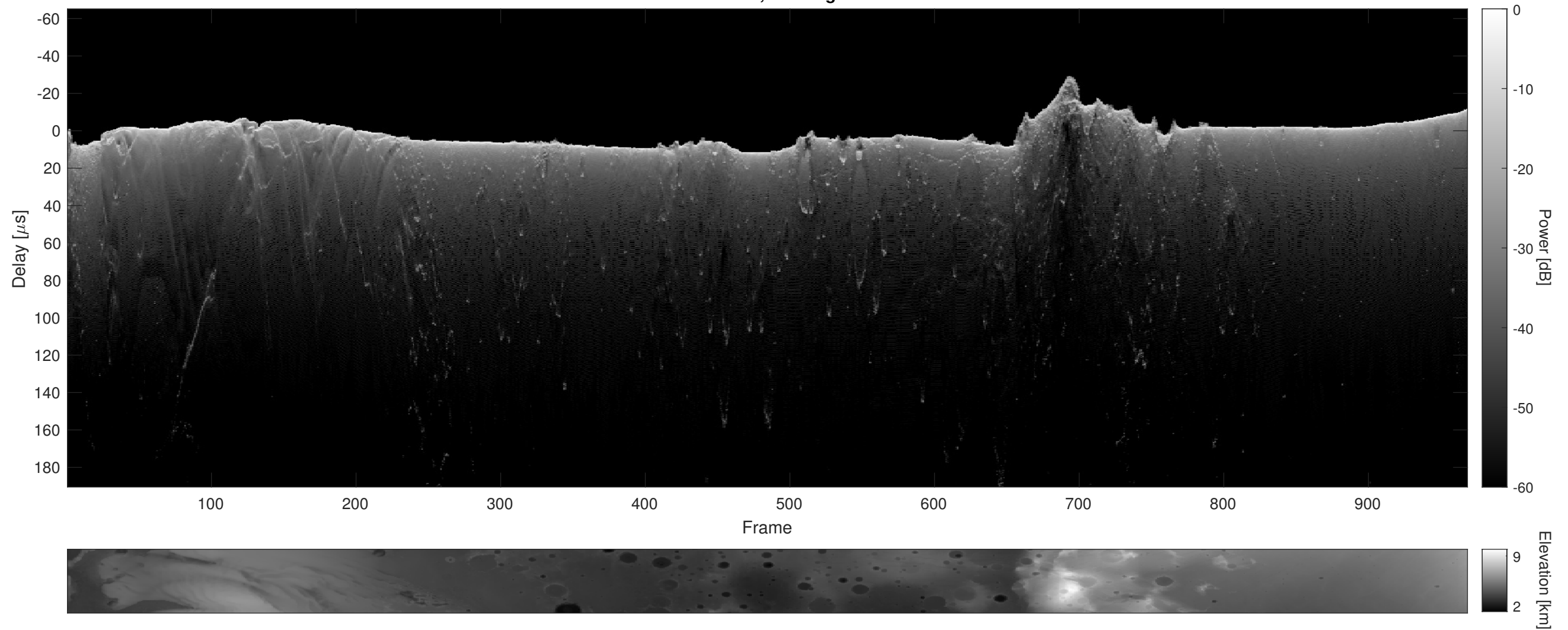
Orbit 12695, Cluttergram
