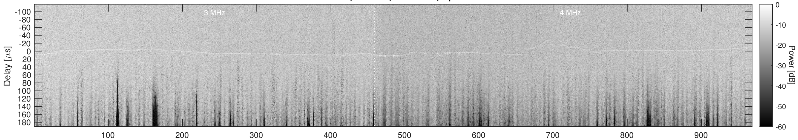
Orbit 12695, Cluttergram
