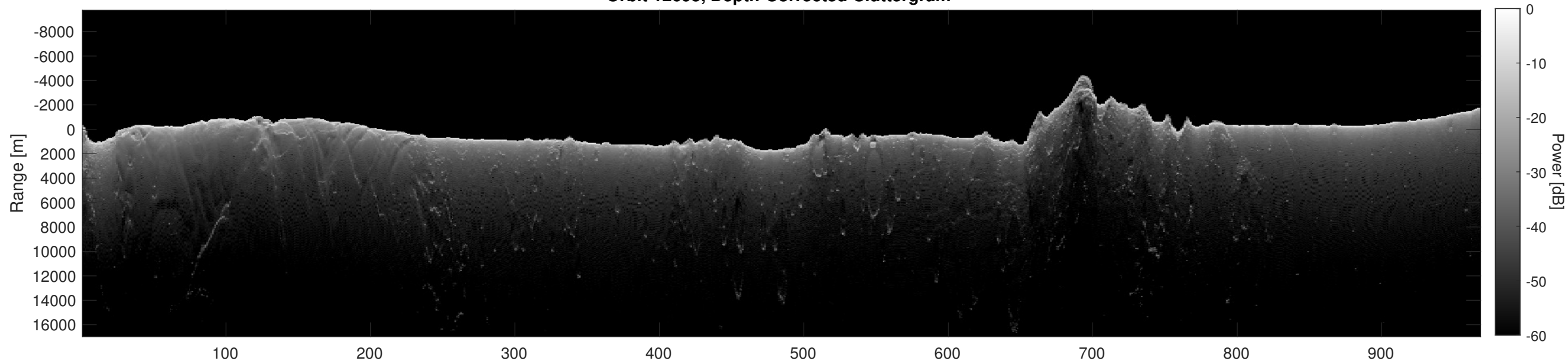
Orbit 12695, Depth-Corrected Cluttergram
