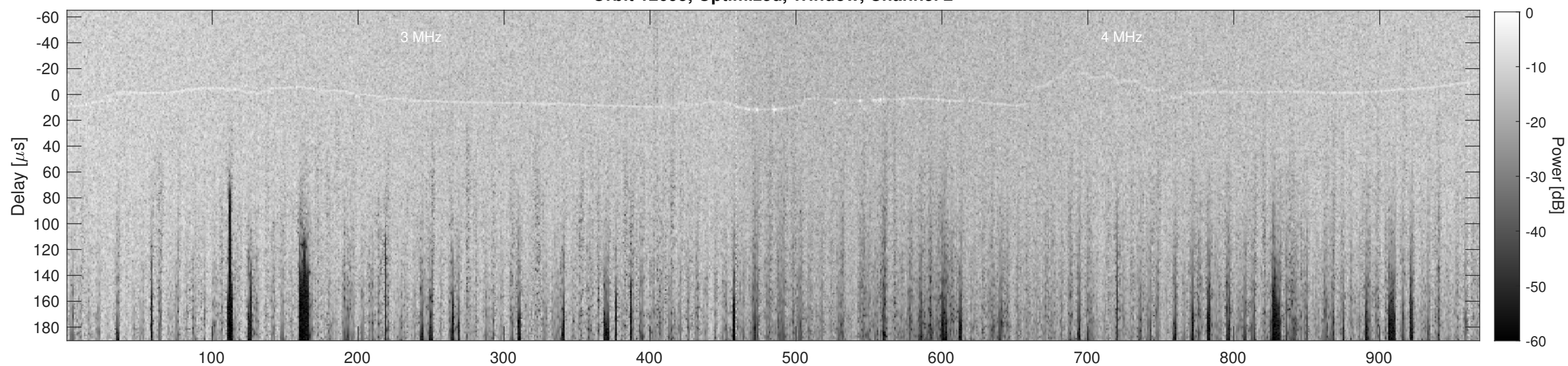
Orbit 12695, Cluttergram
