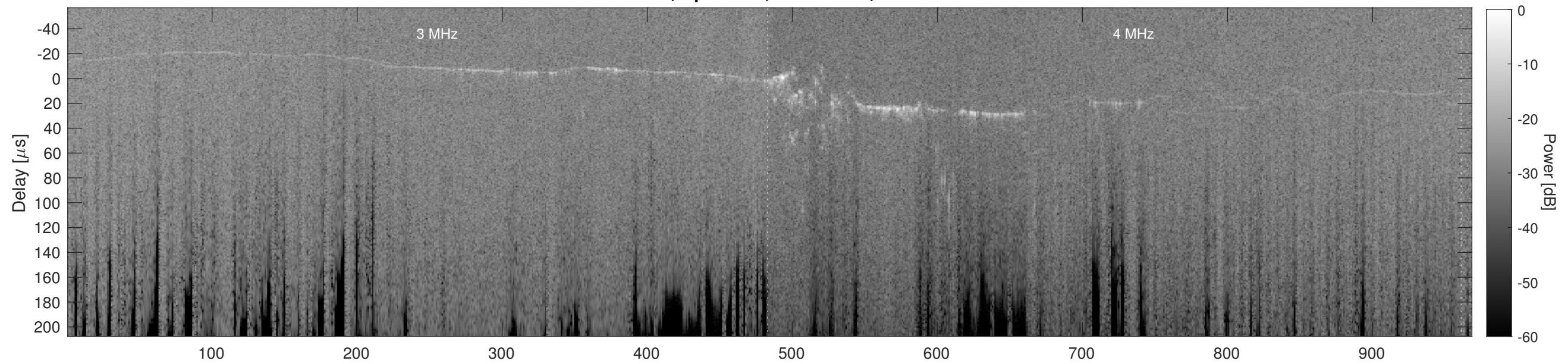
Orbit 12705, Cluttergram
