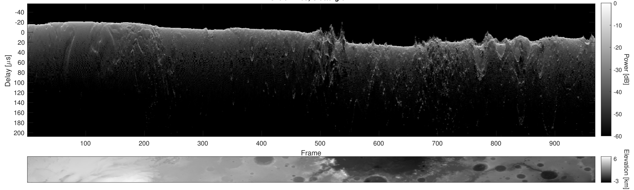
Orbit 12705, Cluttergram
