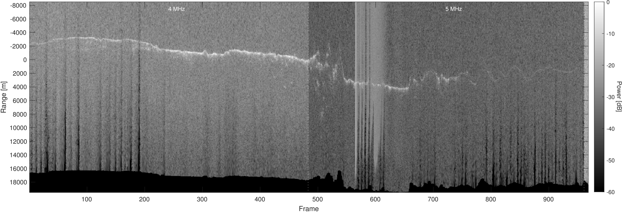
Orbit 12705, Optimized, No Window, Depth-Corrected, Channel 2
