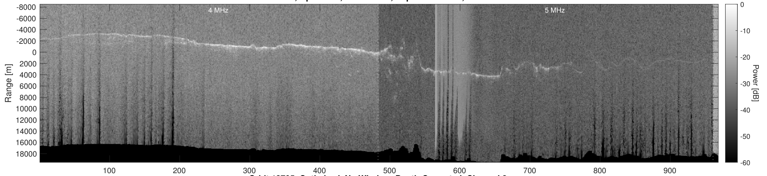
Orbit 12705, Optimized, No Window, Depth-Corrected, Channel 2
