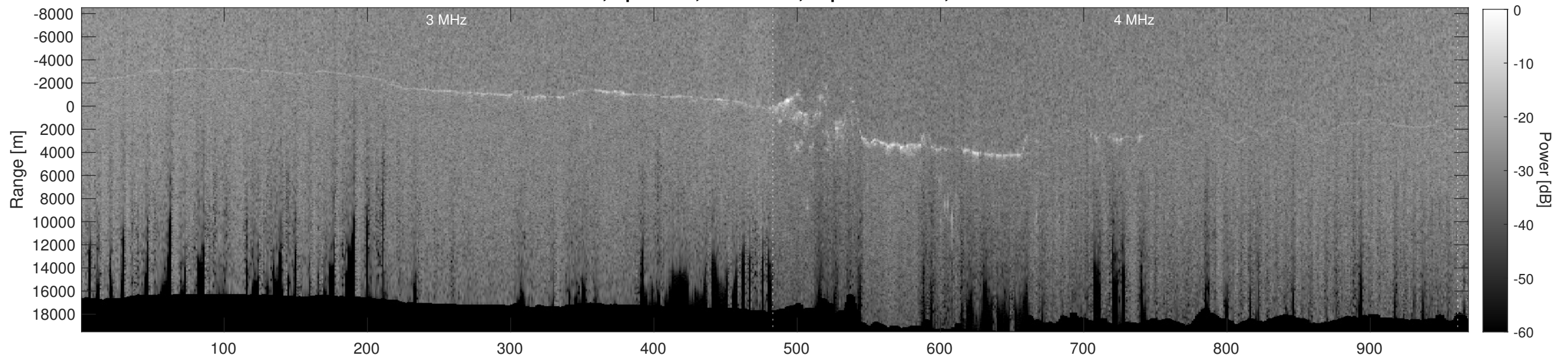
Orbit 12705, Depth-Corrected Cluttergram
