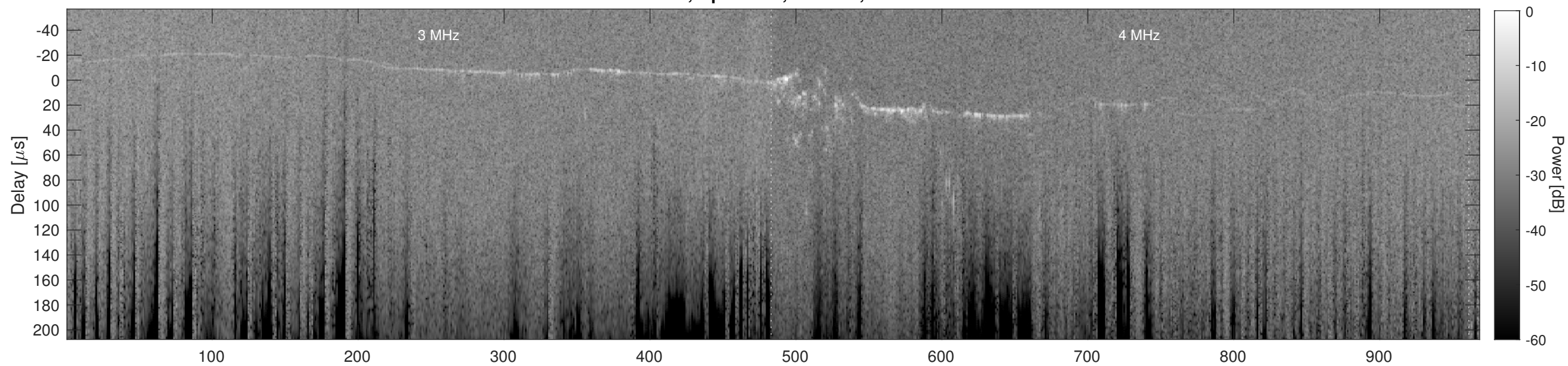
Orbit 12705, Cluttergram
