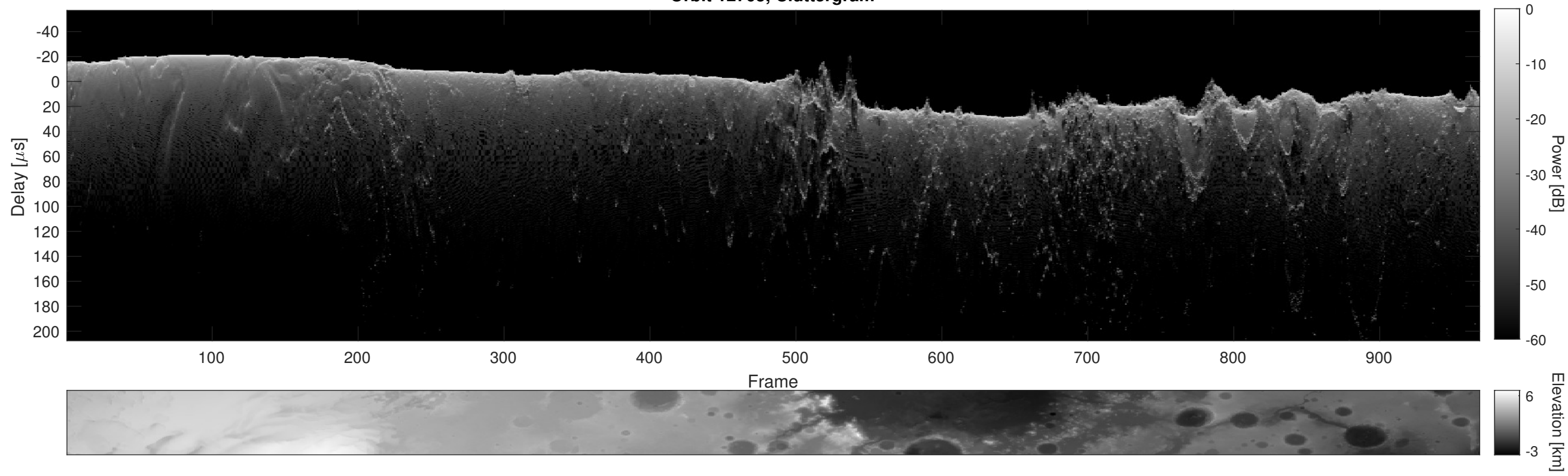
Orbit 12705, Cluttergram
