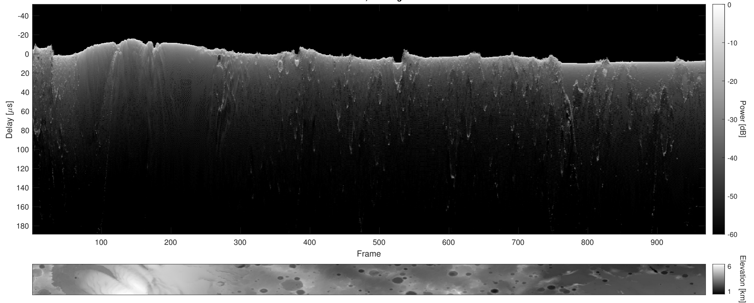
Orbit 12706, Cluttergram
