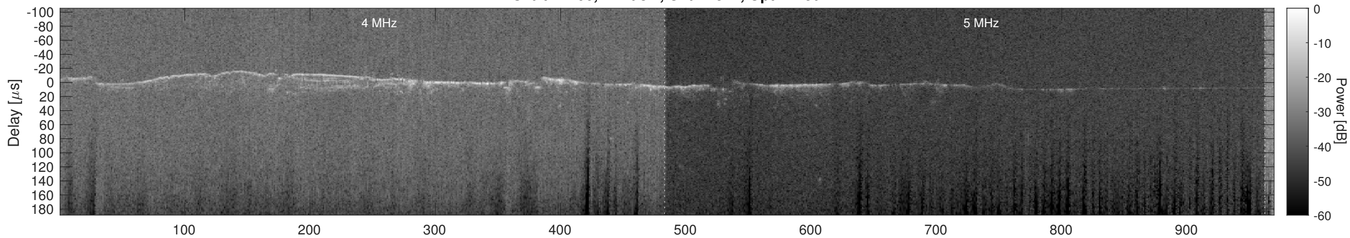
Orbit 12706, Cluttergram
