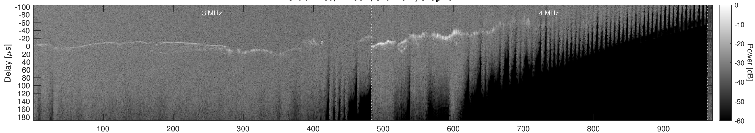
Orbit 12706, Window, Channel 2, Optimized
