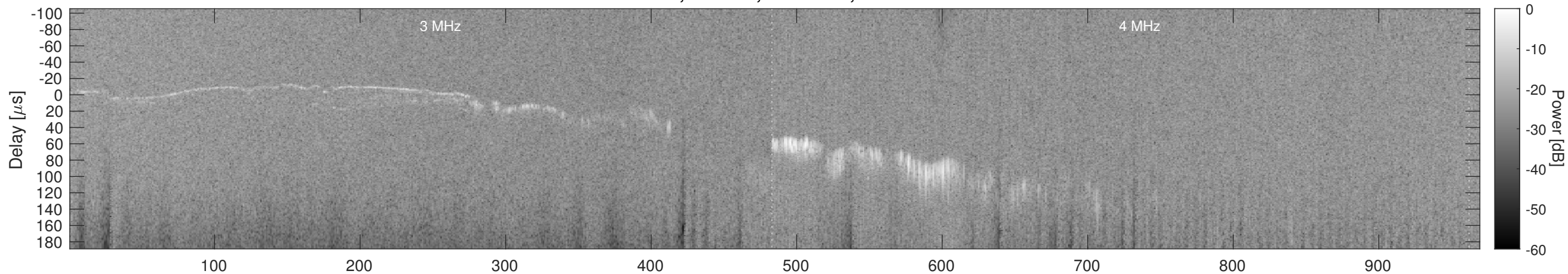
Orbit 12706, Window, Channel 2, Chapman
