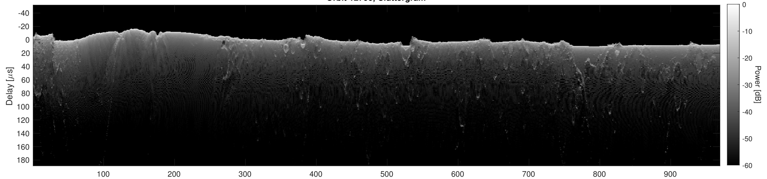
Orbit 12706, Cluttergram
