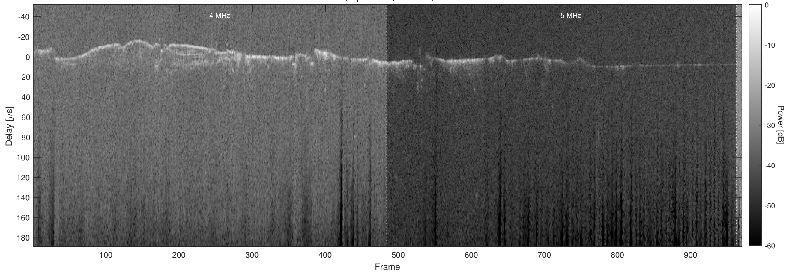
Orbit 12706, Optimized, Window, Channel 2
