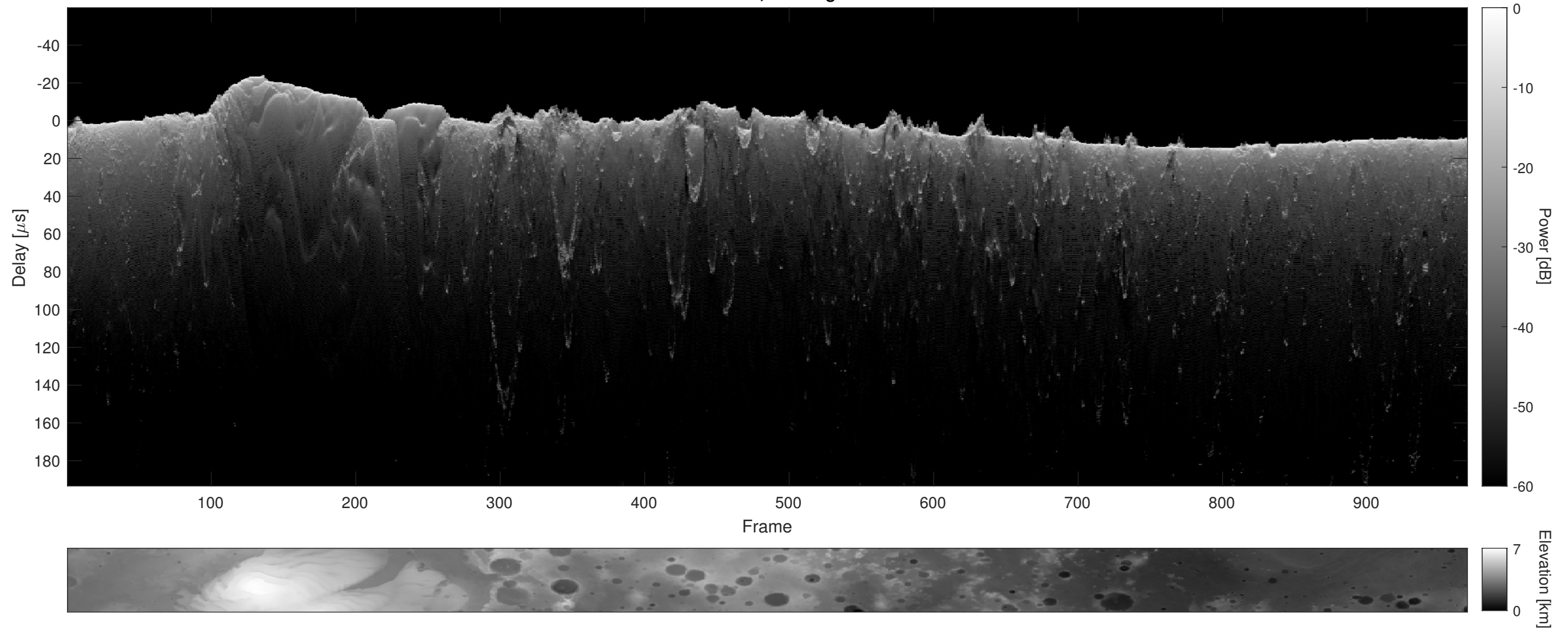
Orbit 12707, Cluttergram
