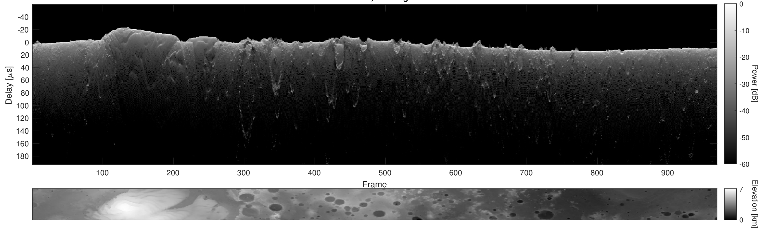
Orbit 12707, Cluttergram
