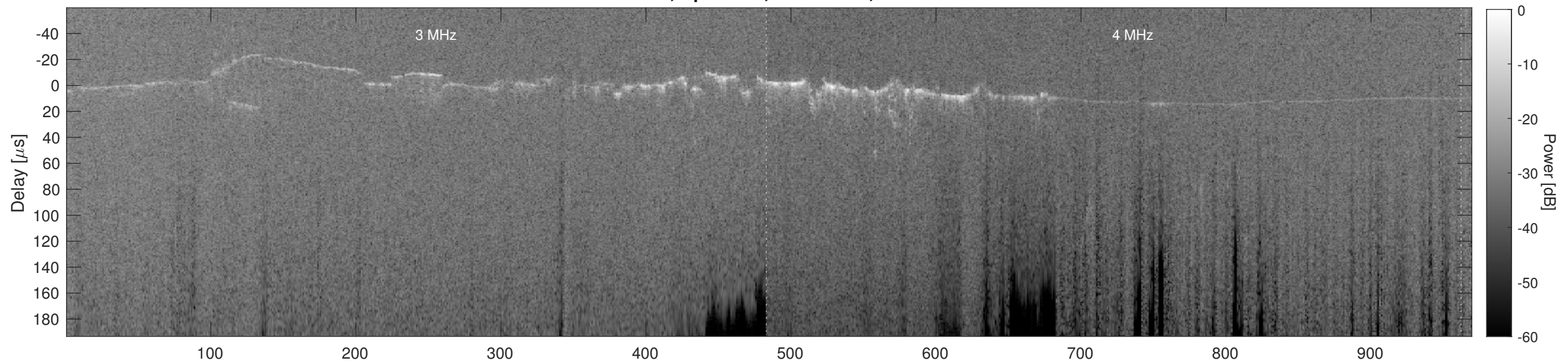
Orbit 12707, Cluttergram
