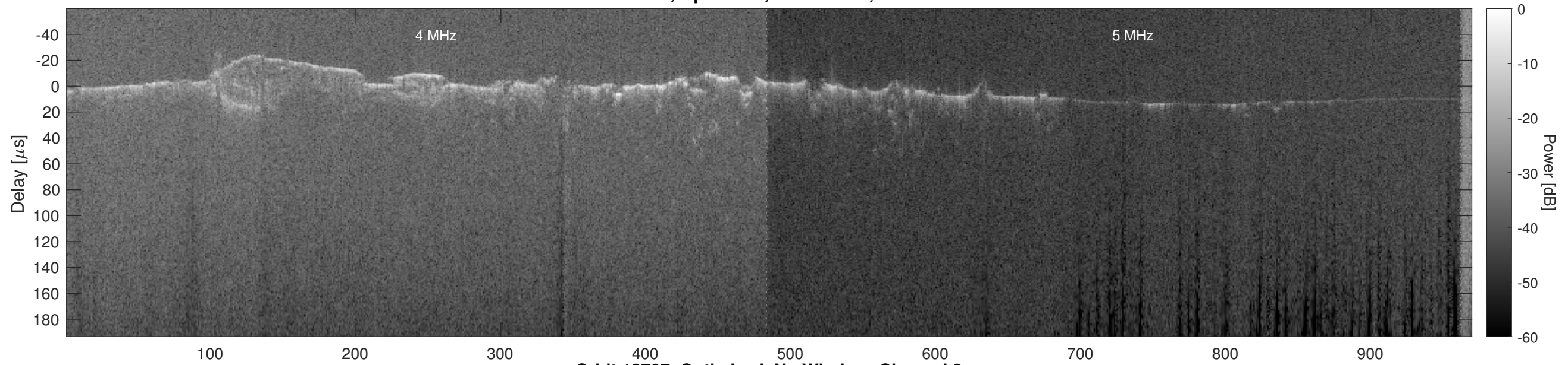
Orbit 12707, Optimized, No Window, Channel 2
