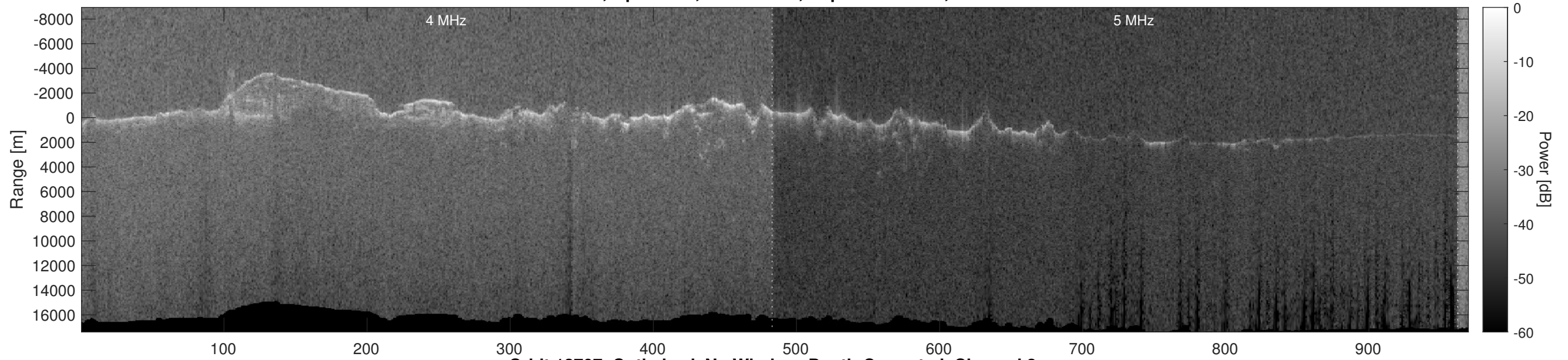
Orbit 12707, Optimized, No Window, Depth-Corrected, Channel 2
