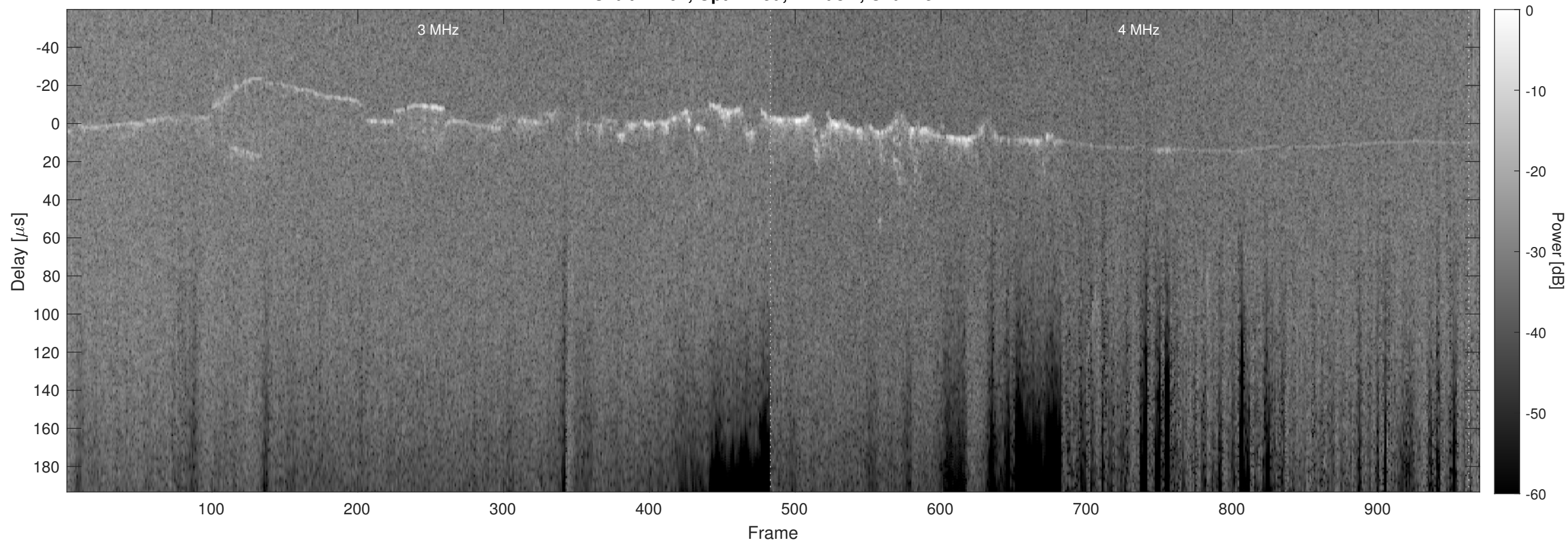
Orbit 12707, Optimized, Window, Channel 2
