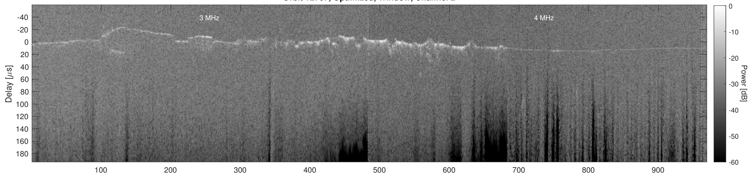
Orbit 12707, Cluttergram
