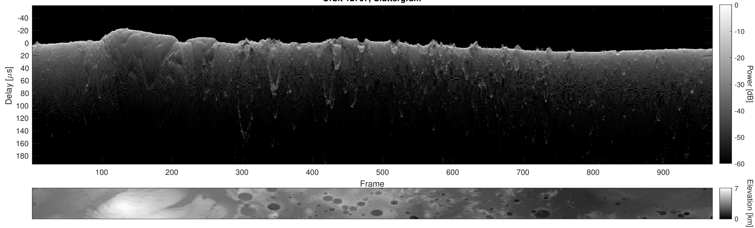
Orbit 12707, Cluttergram
