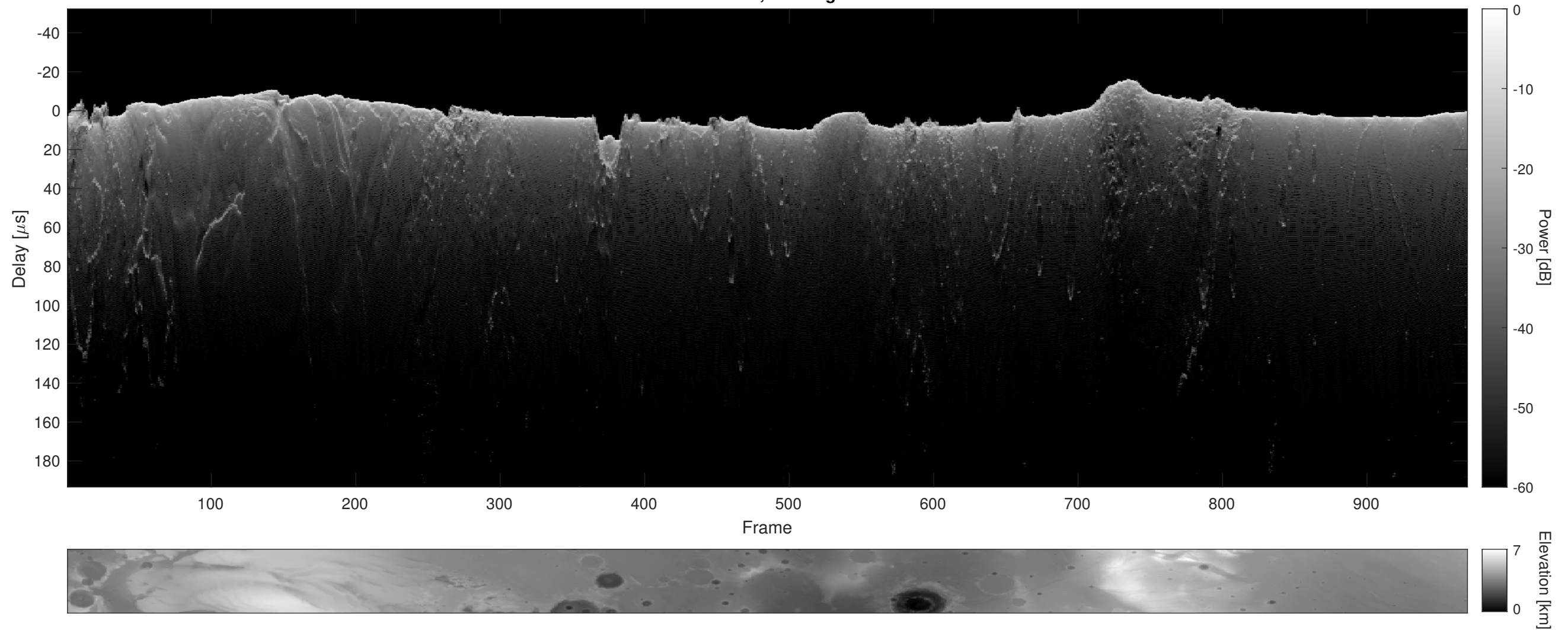
Orbit 12709, Cluttergram
