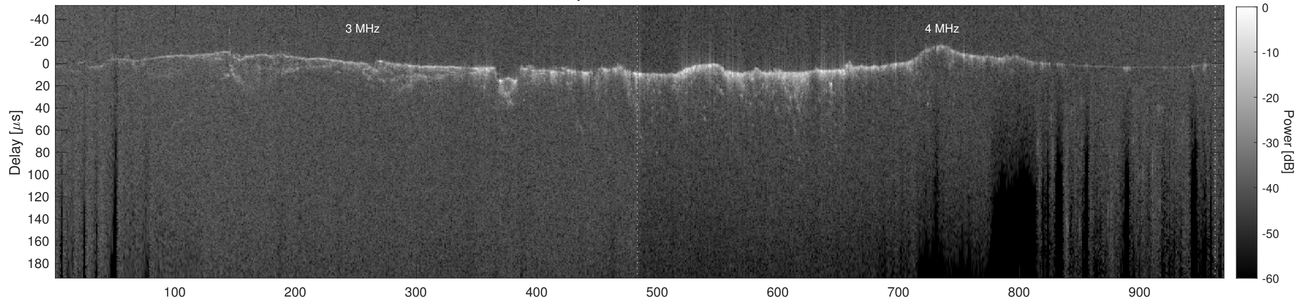
Orbit 12709, Cluttergram
