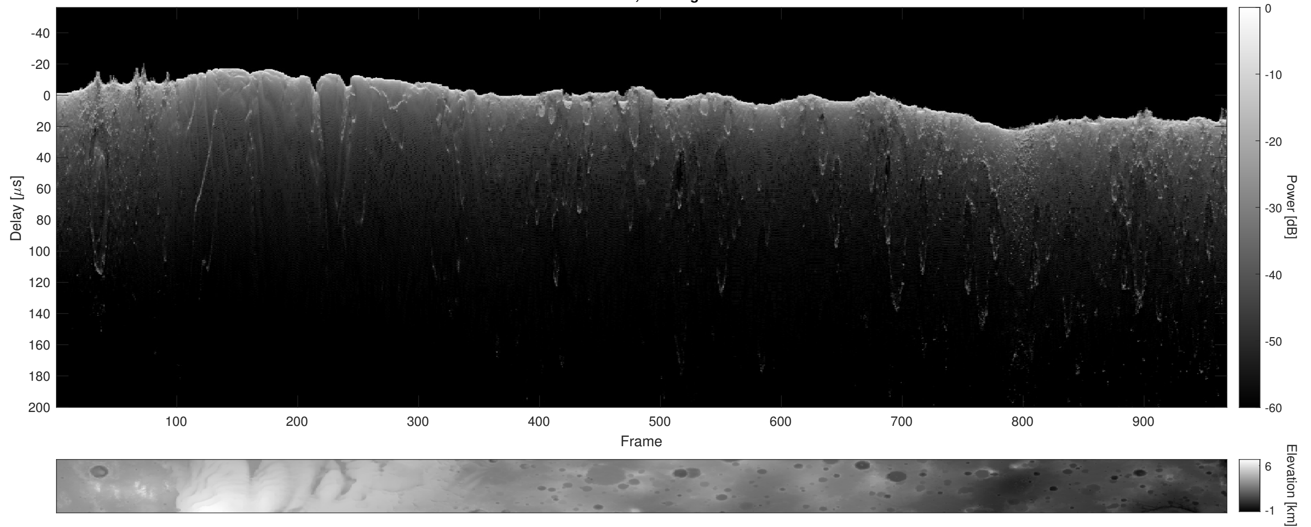
Orbit 12710, Cluttergram
