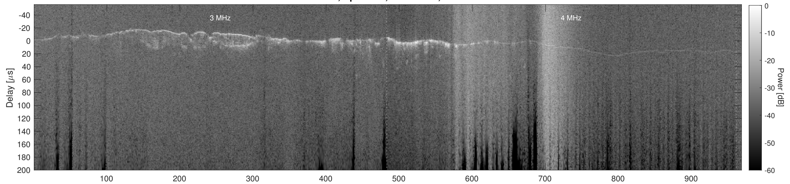
Orbit 12710, Cluttergram
