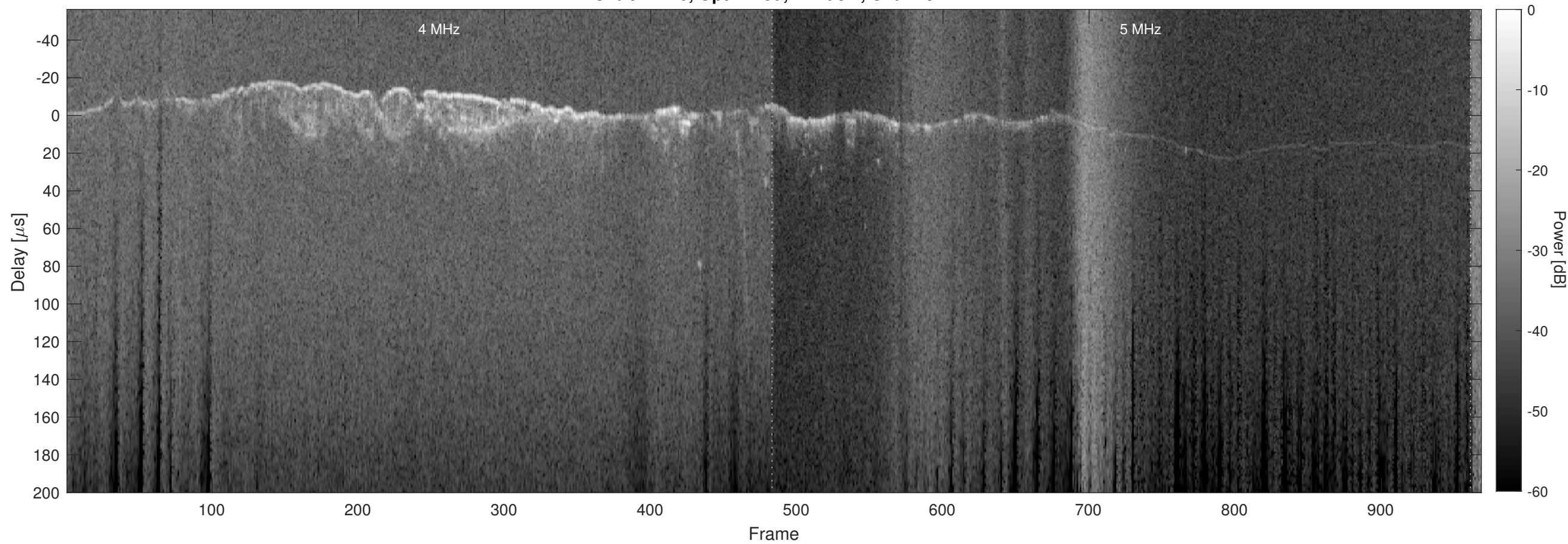
Orbit 12710, Optimized, Window, Channel 2
